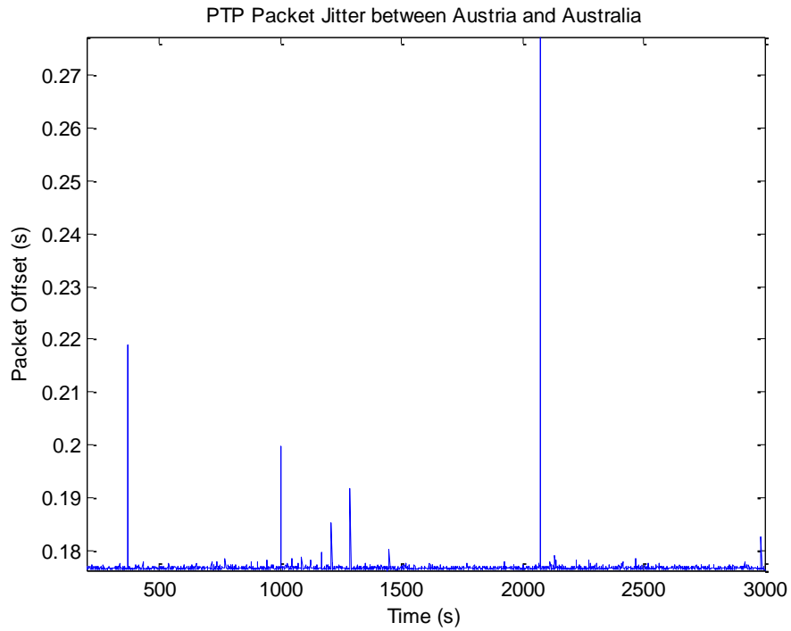
Zoom of the previous figure of packet delay offsets. Samples were taken once a second.
