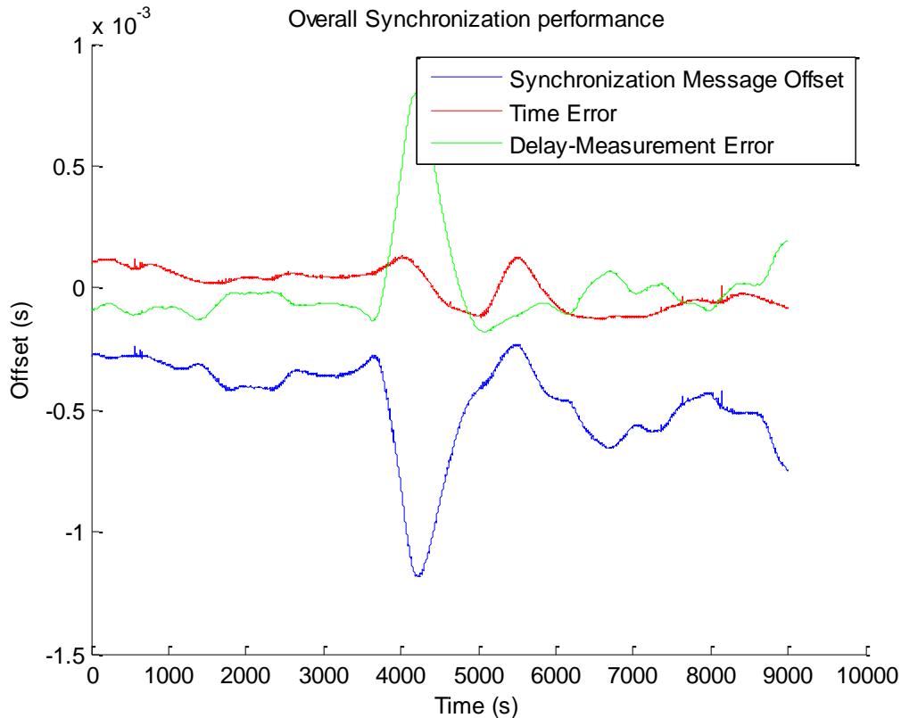
Synchronization performance.
