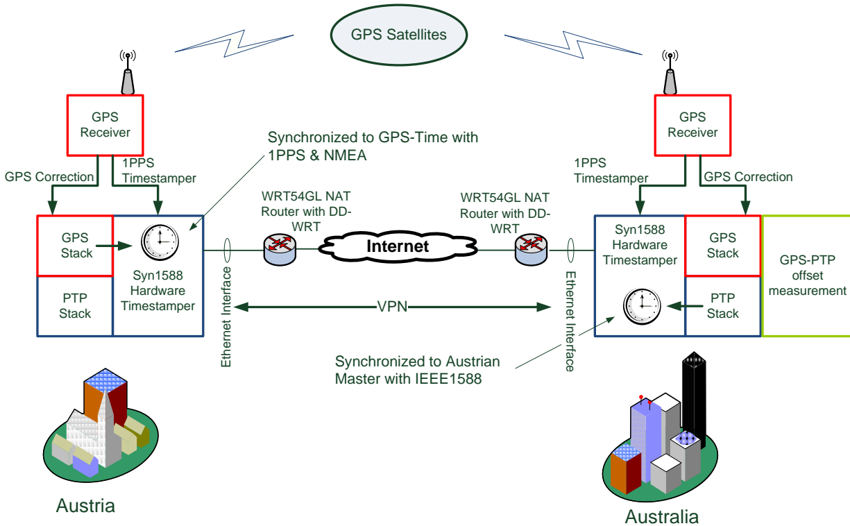
Setup of the test environment.
