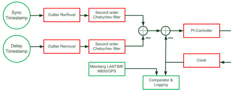
Controller structure.
