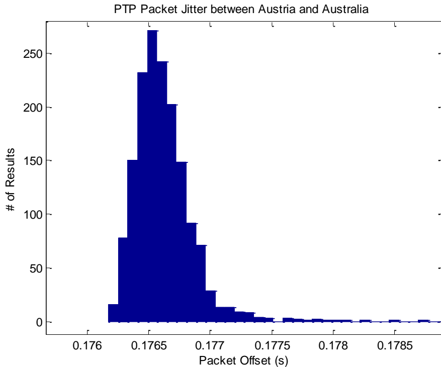
Histogram of the packet offset.
