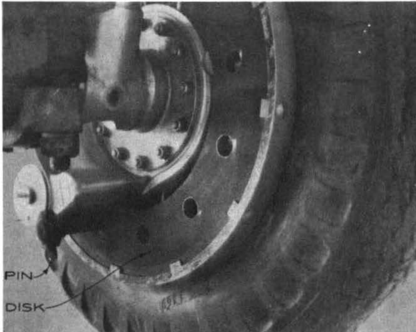
Fig. 2. Soft metal disk and pin improvised for locking wheel on asphaltic concrete
