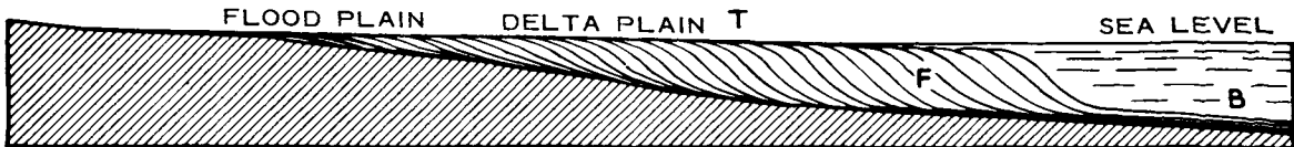
Fig. A1. Section through a delta of the Lake Bonneville type. T, topset beds; F, foreset beds; B, bottomset beds. (After Arthur Holmes, Principles of Physical Geology , The Ronald Press Co., New York, 1945).
