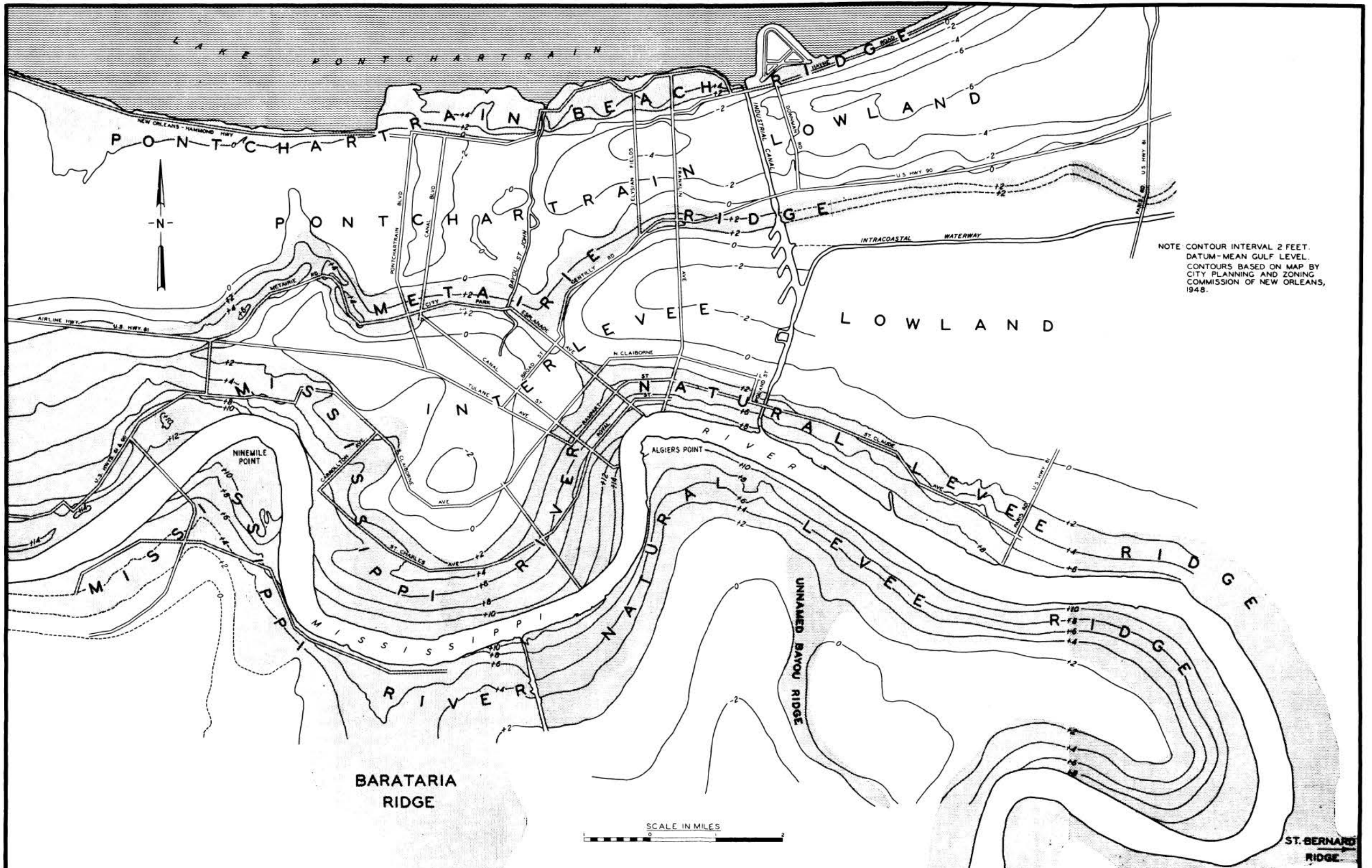
SKETCH SHOWING THE PRINCIPAL PHYSIOGRAPHIC AND TOPOGRAPHIC FEATURES OF THE NEW ORLEANS AREA
