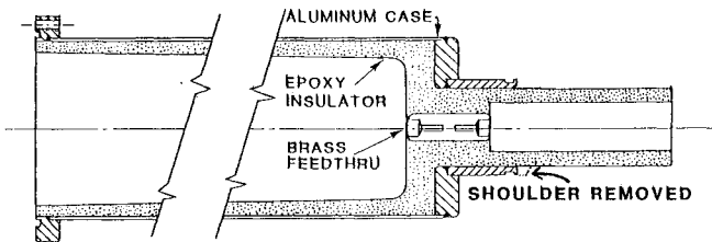
Fig. 5 Section through the housing showing the place where the shoulder was removed.
