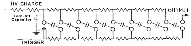
Fig. 7 Schematic diagram of the Marx showing the added turn-off capacitor.
