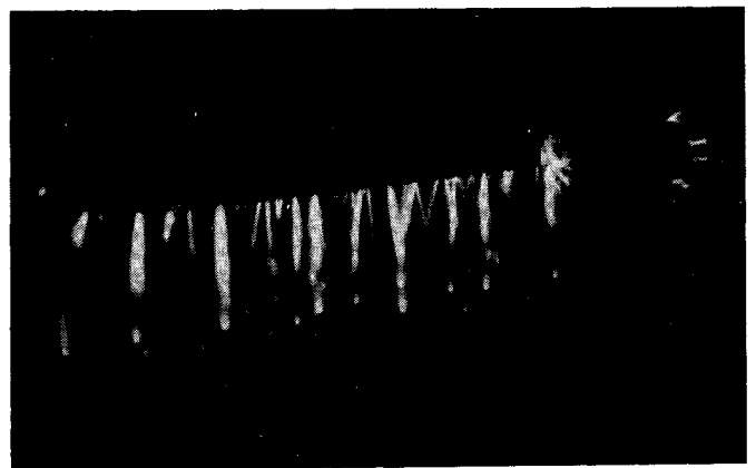
Fig. 8 One shot of the Mini Marx with an 18-inch-long wire three inches above a ground plane plugged into the output. The output insulator is visible on the right.
