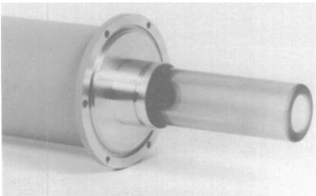
Fig. 6 Photograph of the output insulator of the Marx.
