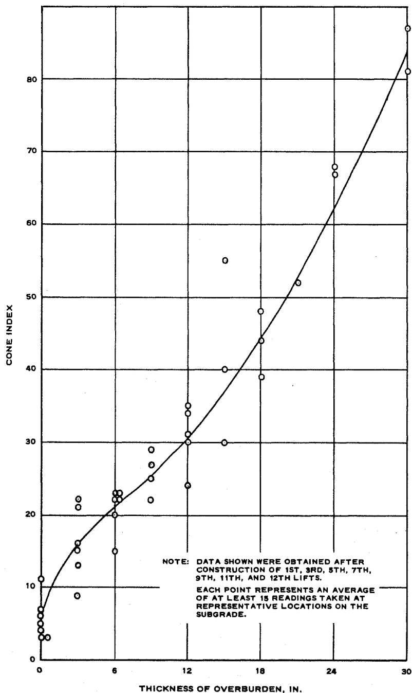
Fig. 8. Relationship of cone index vs thickness of overburden (loess subgrade fill)
