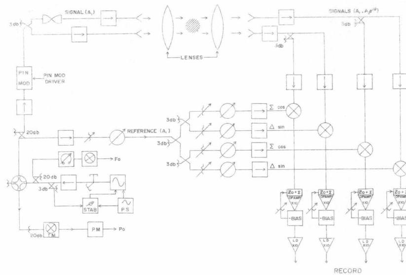
Fig. 4 Block diagram of the X 5 -Band Microwave Interferometer. Transmitter section, lower left; Modulator, Upper left; Horn-Lens systems, upper center; Receiver section, right.
