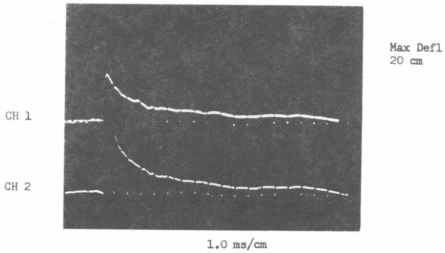
Fig. 22 Typical SIN \phi displays recorded in the wake of a 2.7 in. dia. sphere launched at 14,500 ft/sec in air at 10 torr.
