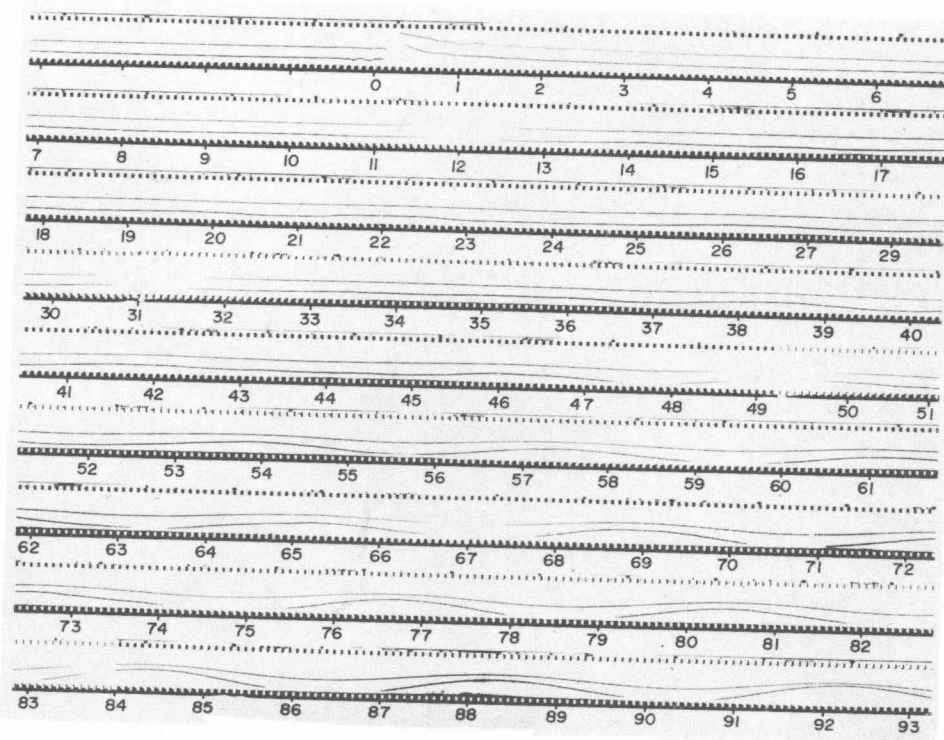
Fig. 29 Fastax film illustrating the long-wave periodic modulation disturbance of the interferometer signals due to the effect of mechanical vibration following the launching of a projectile.
