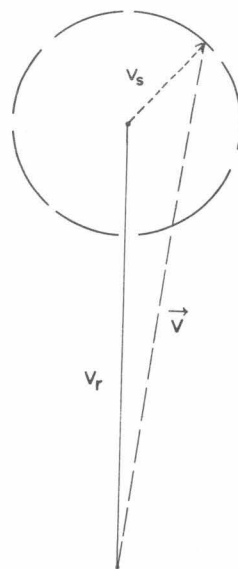
Fig. 17 Vector relationship illustrating that the reference signal is made much greater than the transmitted signal (In terms of power, the reference signal is made 100 times the level of the transmitted signal).
