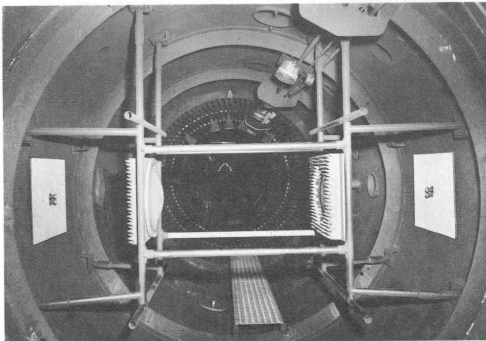
Fig. 5 Wide-angle photograph of the range interior at the Interferometric Station 272 showing transmitter antenna (left) the double focussing lens system (center), and the receiving antenna (right). The focussing lens (right) is partially obscured by E & C CV-4 microwave absorber.
