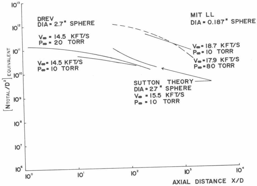
Fig. 27 Comparison of DREV and MIT LL exponential electron density decay in a sphere wake. Also shown are theoretical results calculated by Sutton.
