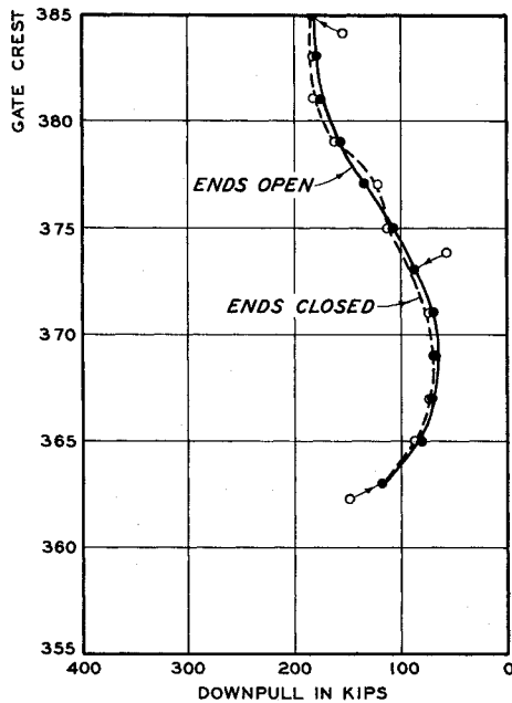
TAILWATER ELEVATION 373.0
