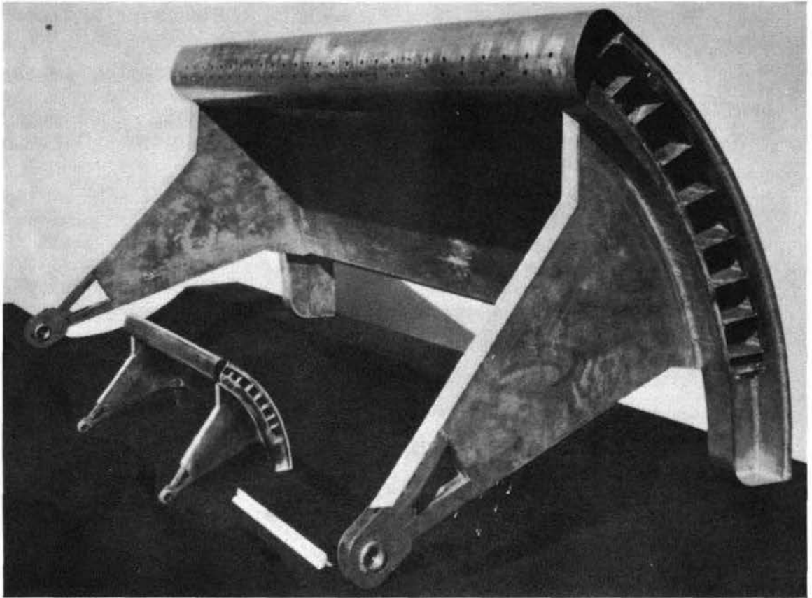
Fig. 8. 1:36- and 1:10-scale models of the plan 2, alternate E gate
