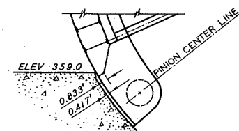
MODIFICATION AT BOTTOM OF GATE
