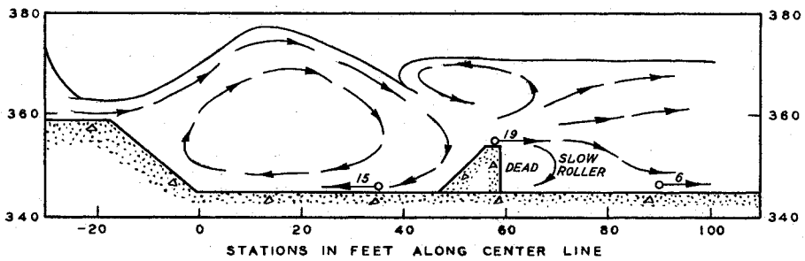
END SILL AT STATION 0+59
