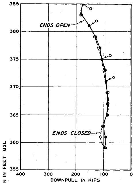
TAILWATER ELEVATION 381.0
