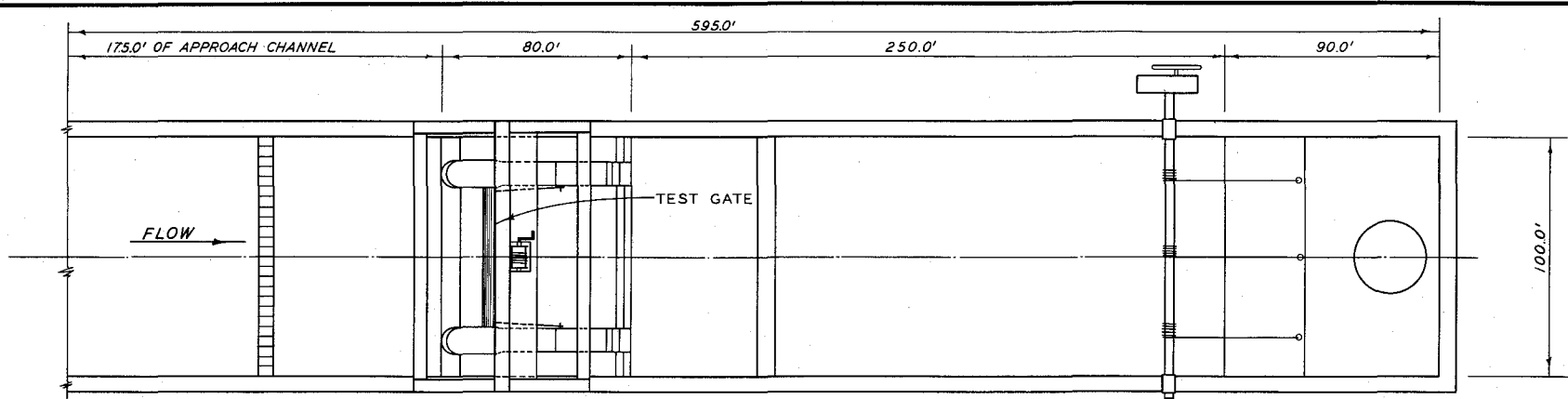
PLAN
