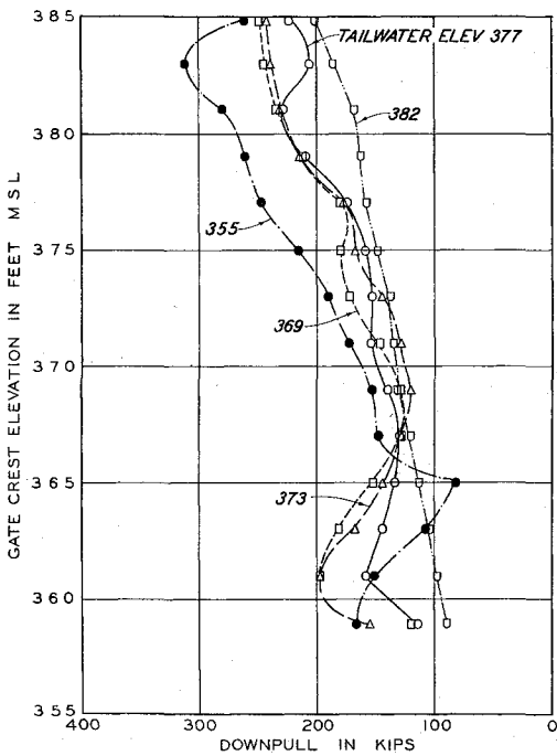
RAISING GATE - POOL ELEVATION 382.0
