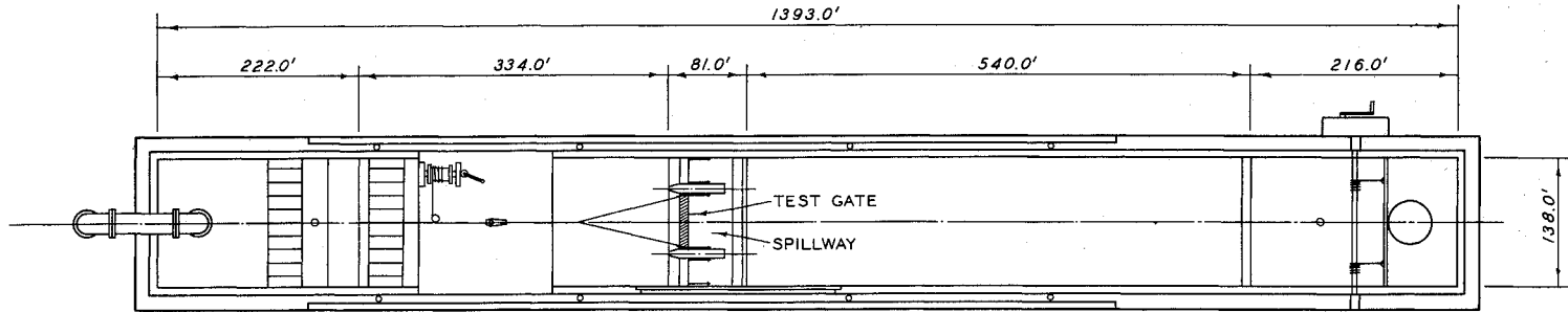
PLAN
