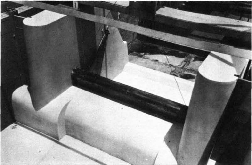
Fig. 4. Downstream view, 1:10-scale model, revised design (plan 2)
