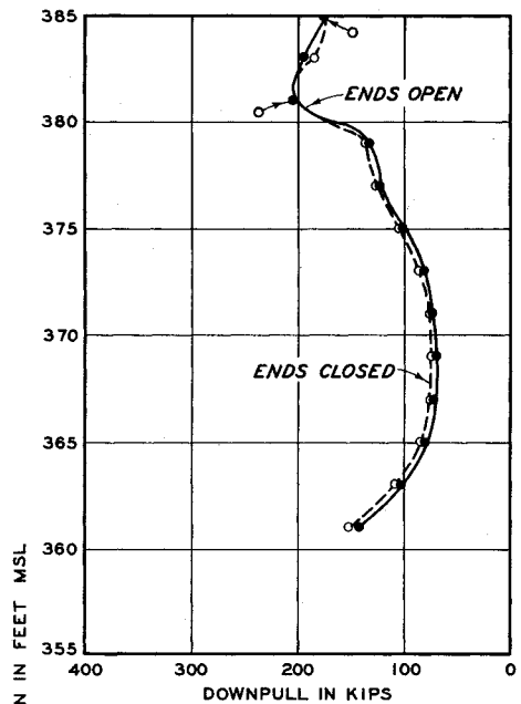
TAILWATER ELEVATION 377.0
