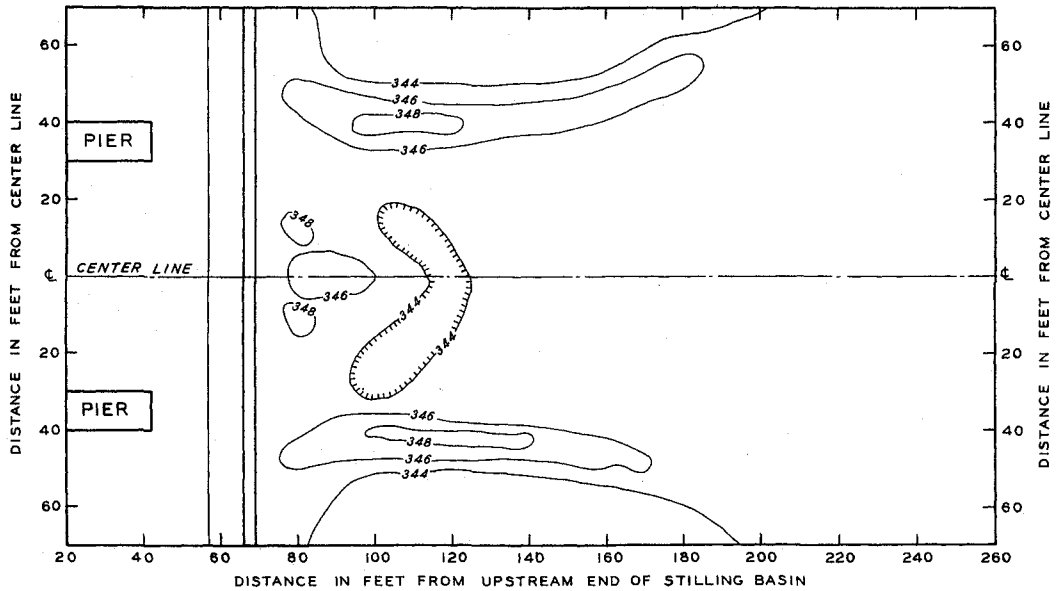
9-FT END SILL AT STATION 0+69
