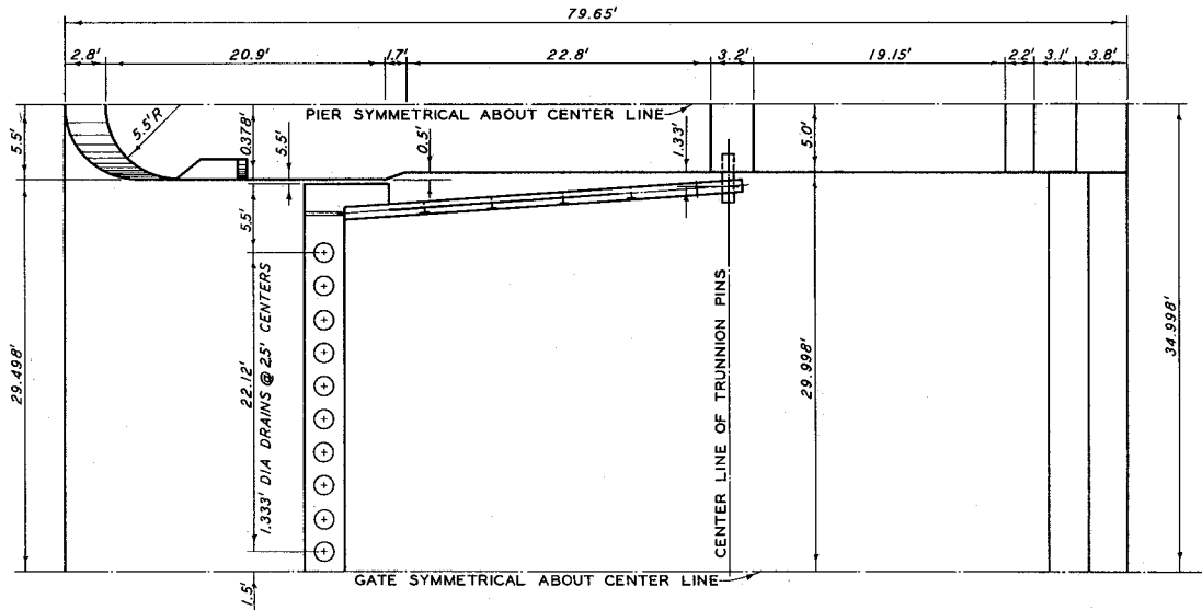
HALF PLAN
