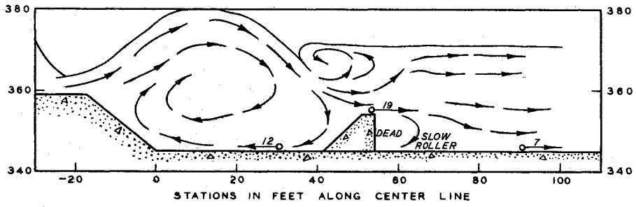
END SILL AT STATION 0+54
