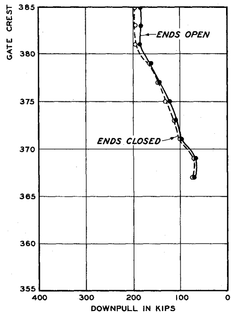
TAILWATER ELEVATION 369.0
