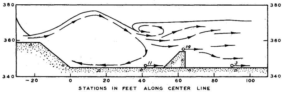
END SILL AT STATION 0+64
