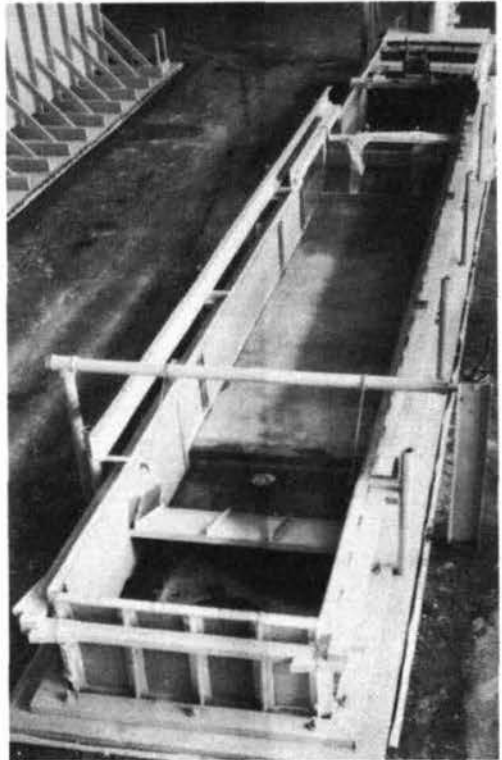
Fig. 2. Upstream view, 1:36-scale model, original design
