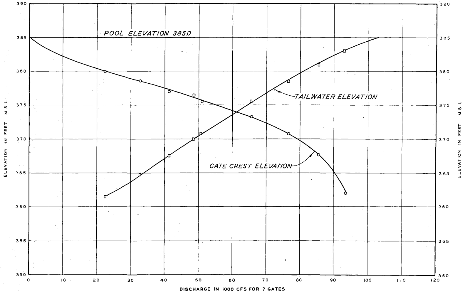
RATING CURVE GATE OPENING VS POOL AND TAILWATER ELEV PLAN 2 GATE
