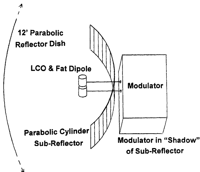
Figure 4. Schematic of the LCO transmitter.
