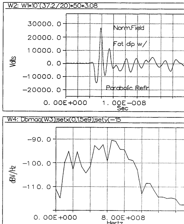
Figure 7. Received E-field and frequency spectrum for the 700 MHz LCO.
