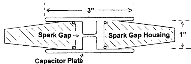
Figure 1. 700 MHz LCO cross-section showing the two capacitor plates, insulator, and switch.
