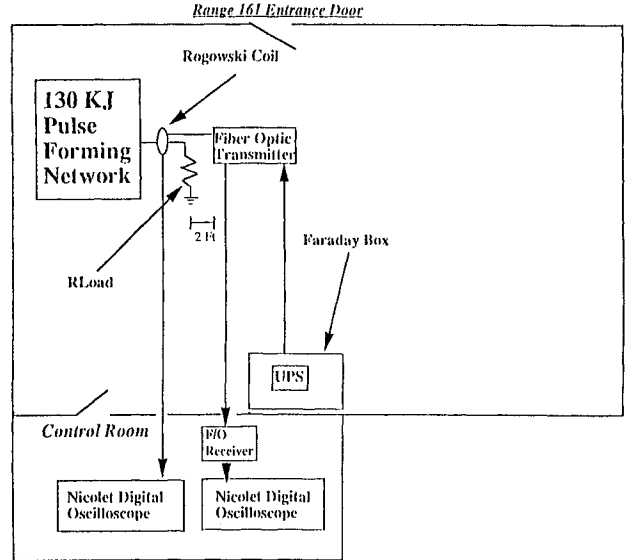
Figure 6. Experimental Setup for Test No. 2.
