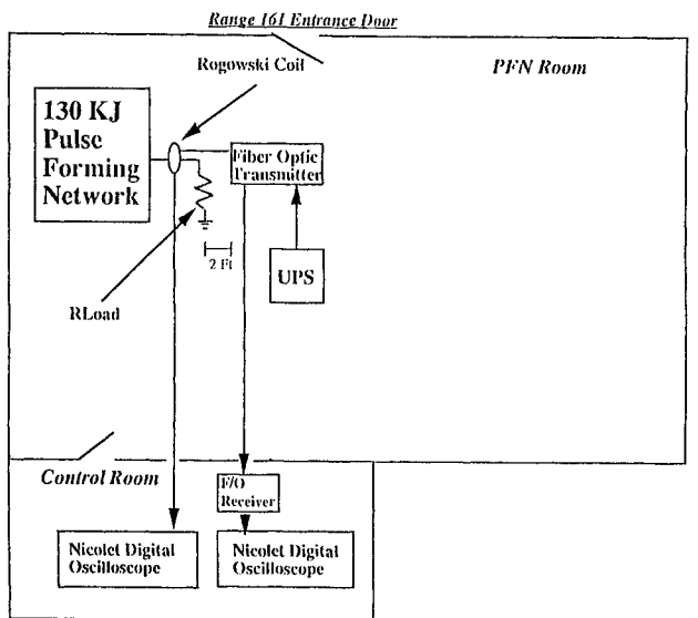
Figure 8. Experimental Setup for Test No. 3.
