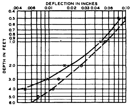
250-SQ-IN. PLATE - DUAL SPACING 2.5 FT
