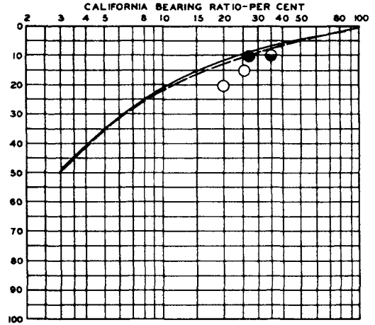
B-29 ASSEMBLY LOAD OF 70,000 LB
