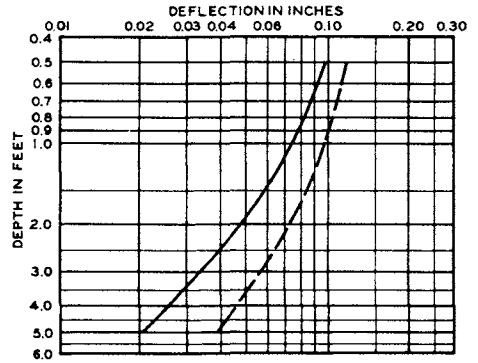
500-SQ-IN. PLATE - DUAL SPACING 3.0 FT
