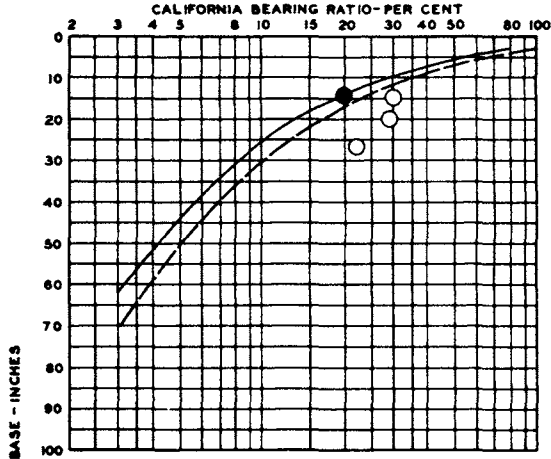
B-36 ASSEMBLY LOAD OF 150,000 LB
