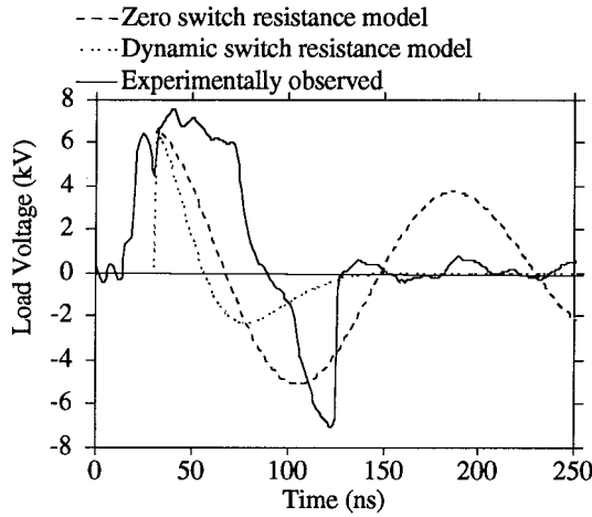
Figure 5. Computer model and experimental result of the switch behavior in the circuit of Fig. 3 when operated at a charging voltage of V_o = 6.7\text{-kV} .
