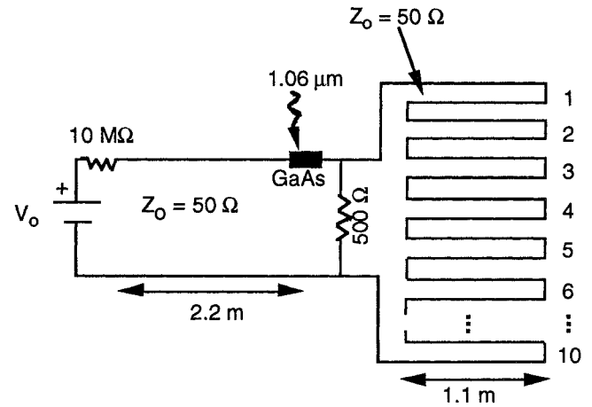
Figure 3. Inductive energy storage pulsed power system (IESPPS) with 500- \Omega characteristic impedance constructed from ten 50- \Omega CCTL's placed in series with floating shields.
