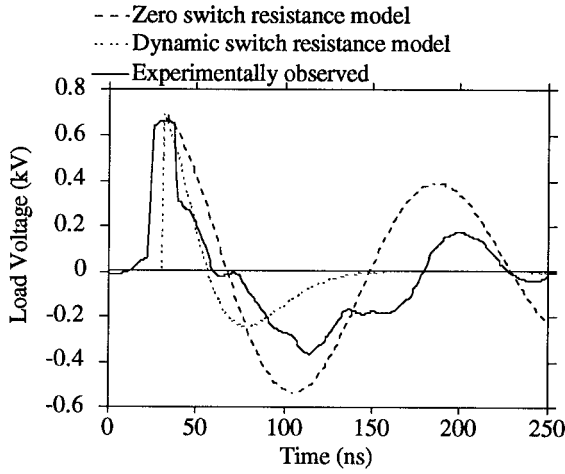
Figure 4. Computer model and experimental result of the switch behavior in the circuit of Figure 3 when operated at a charging voltage of V_o = 700\text{-V} .
