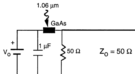
Figure 1. Basic current charged transmission line (CCTL) circuit.
