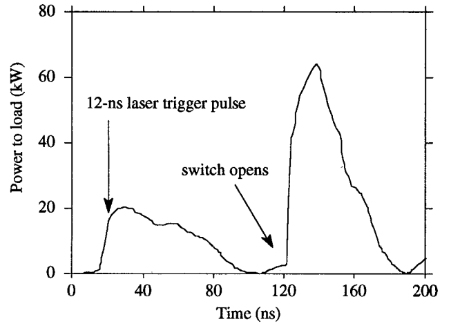
Figure 6. 5-mm cube GaAs switch operated in the circuit of Fig. 3 with V_o = 3.8\text{-kV} .
