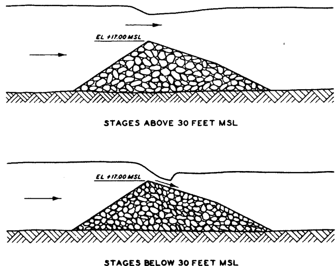
Fig. 3. Water-surface profiles over the rock fill for the Mississippi River stages indicated
