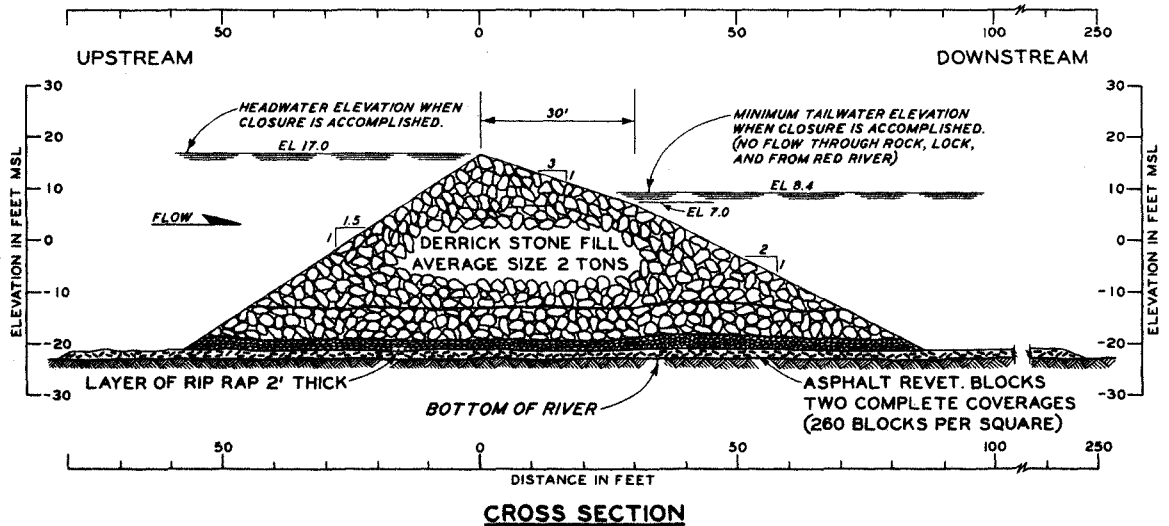
Fig. 2. Proposed design for the rock fill
