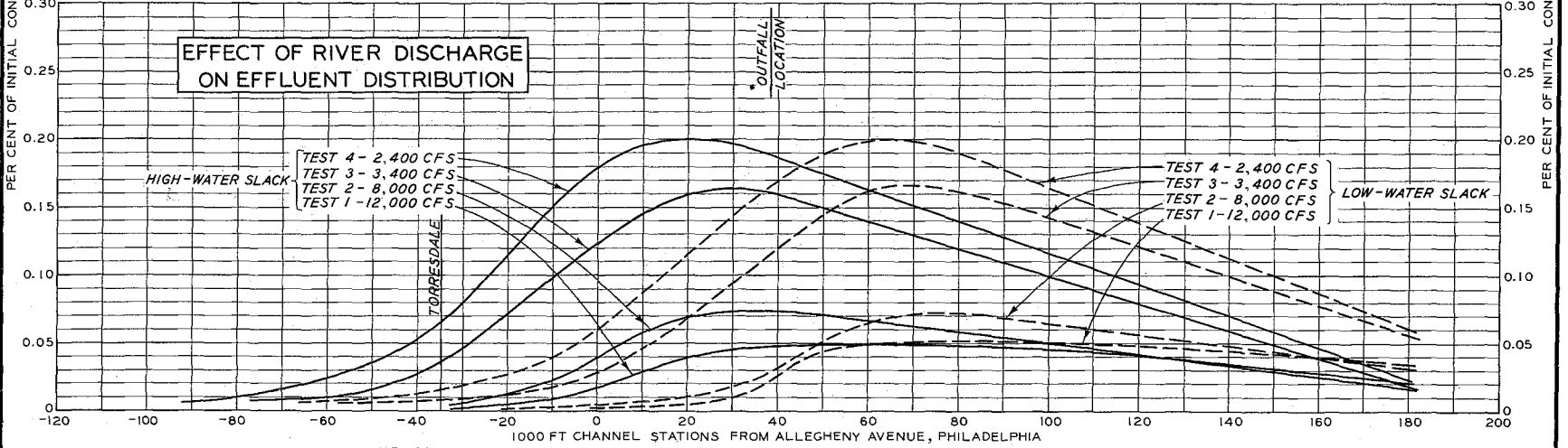
EFFECT OF MODE OF PLANT DISCHARGE AND EFFECT OF RIVER DISCHARGE ON EFFLUENT DISTRIBUTION
