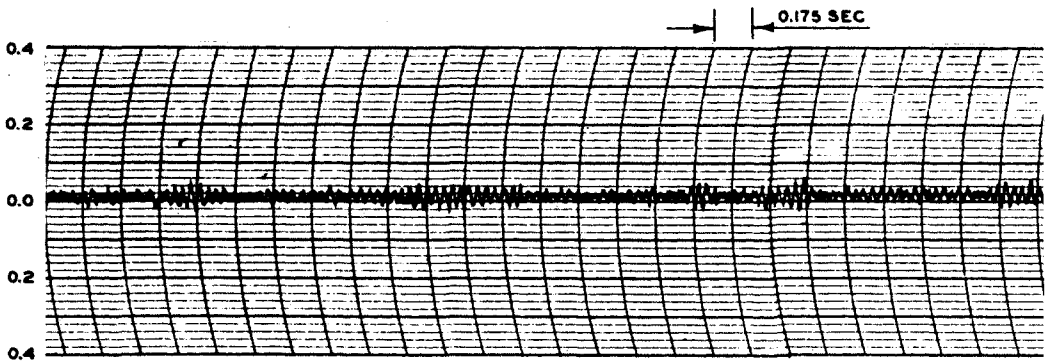
VERTICAL VIBRATION
