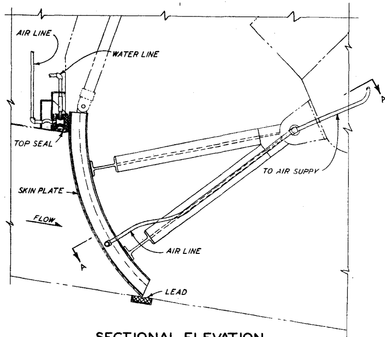
SECTIONAL ELEVATION
