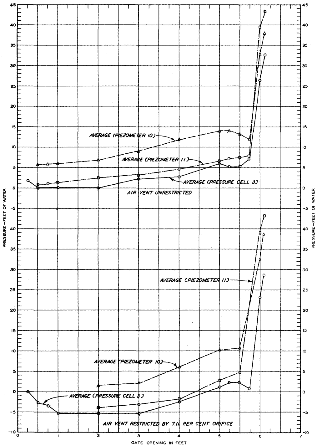
PRESSURE COMPARISONS PRESSURE CELL 3 PIEZOMETERS 10 AND 11
