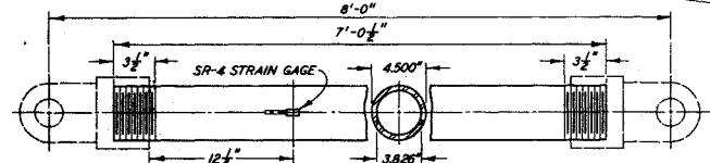
DETAILS OF LIFTING STRUT
