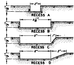
DETAILS OF TEST RECESSES
