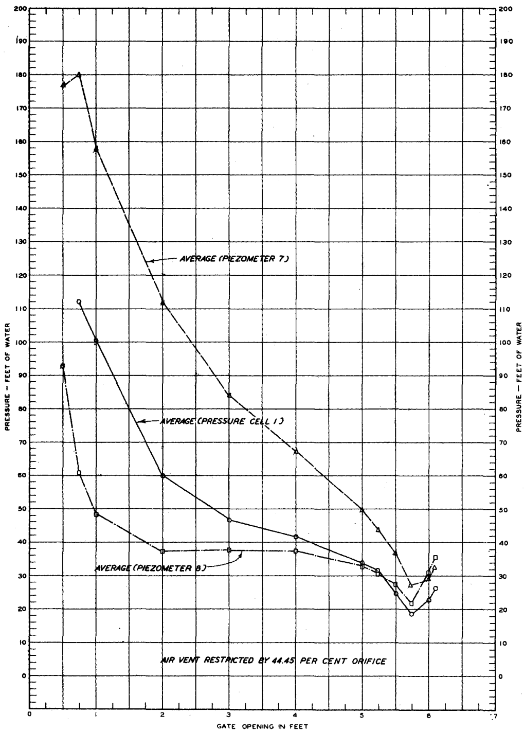
PRESSURE COMPARISONS PRESSURE CELL 1 PIEZOMETERS 7 AND 8
