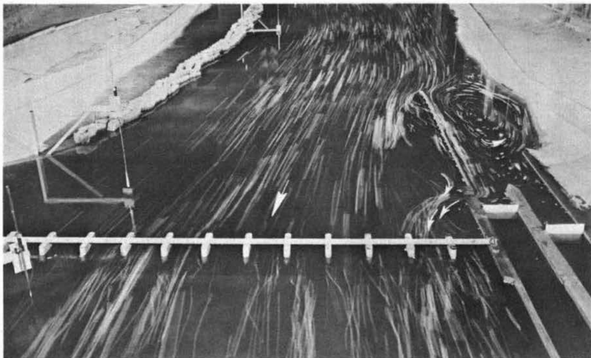
Photograph 31. Plan C: surface currents in upper lock approach with 27 ports and 50-ft ice and drift chute in upper guard wall. Discharge, 500,000 cfs
