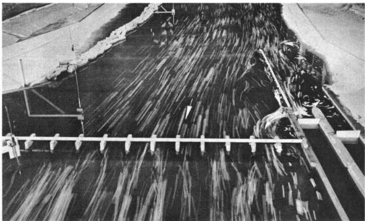
Photograph 30. Plan C: surface currents in upper lock approach with 27 ports and 50-ft ice and drift chute in upper guard wall. Discharge, 420,000 cfs
