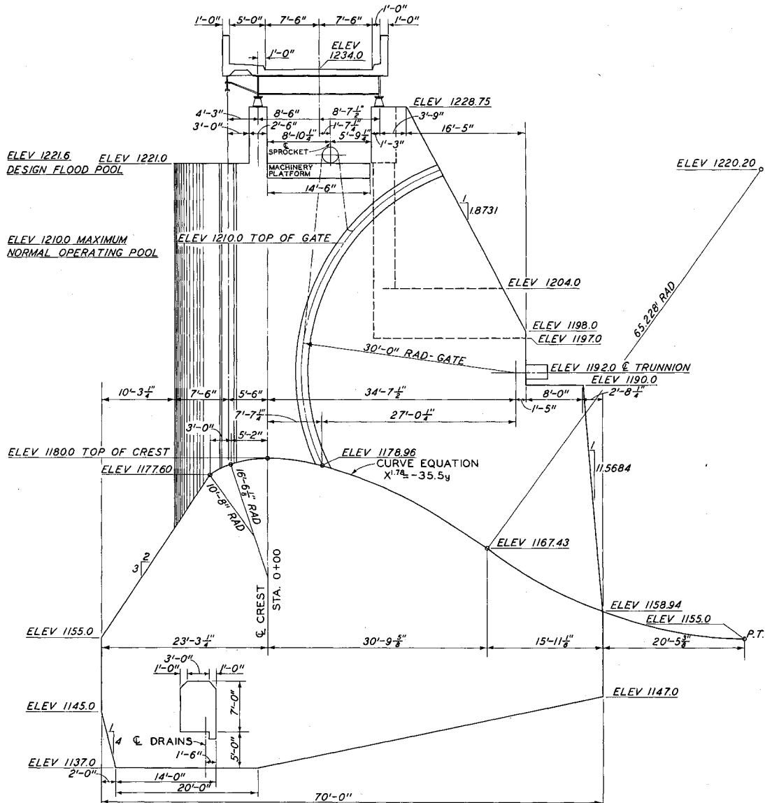
SPILLWAY ELEVATION
