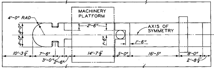
PLAN (BRIDGE NOT SHOWN)
