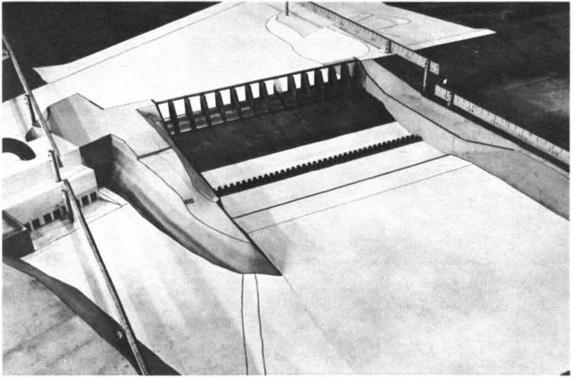
Upstream view
