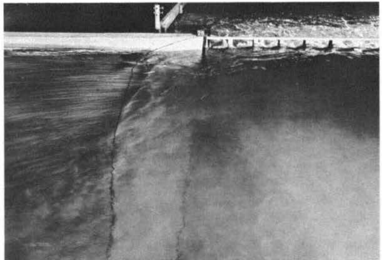
Fig. 3. Flow at left abutment, original design
