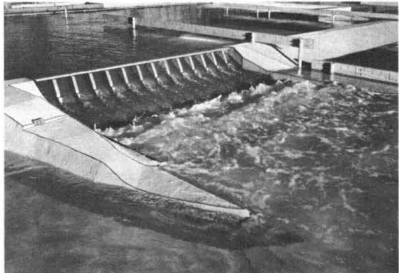
Fig. 8. Original design stilling basin
