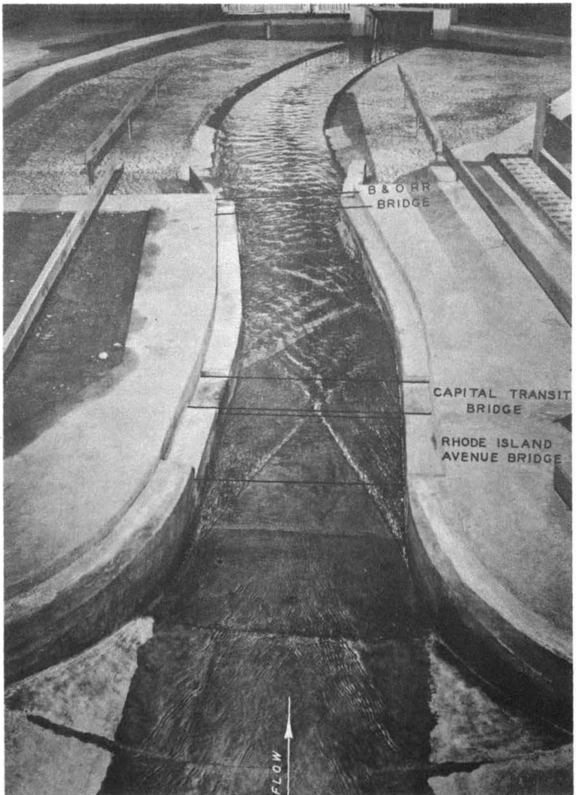
Photograph 15. Plan C: flow conditions from upstream end of paved channel to lower end of model. Discharge, 2000 cfs; tailwater elevation, 4.0 ft msl
