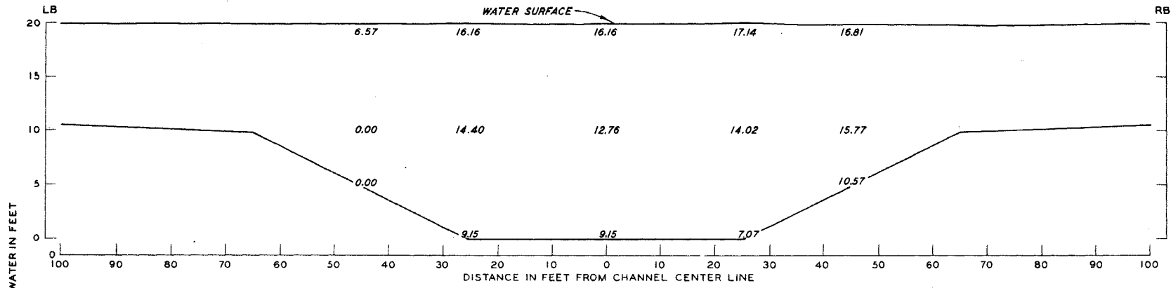
STATION 11+15
