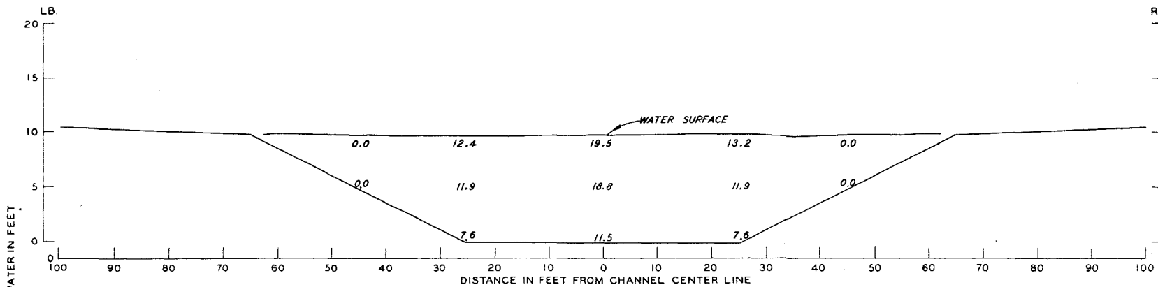
STATION 11+15
