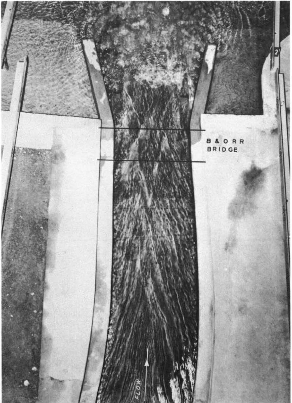
Photograph 10. Plan C: position of hydraulic jump below the Baltimore and Ohio Railroad bridge. Discharge, 20,000 cfs; tailwater elevation, 15.4 ft msl
