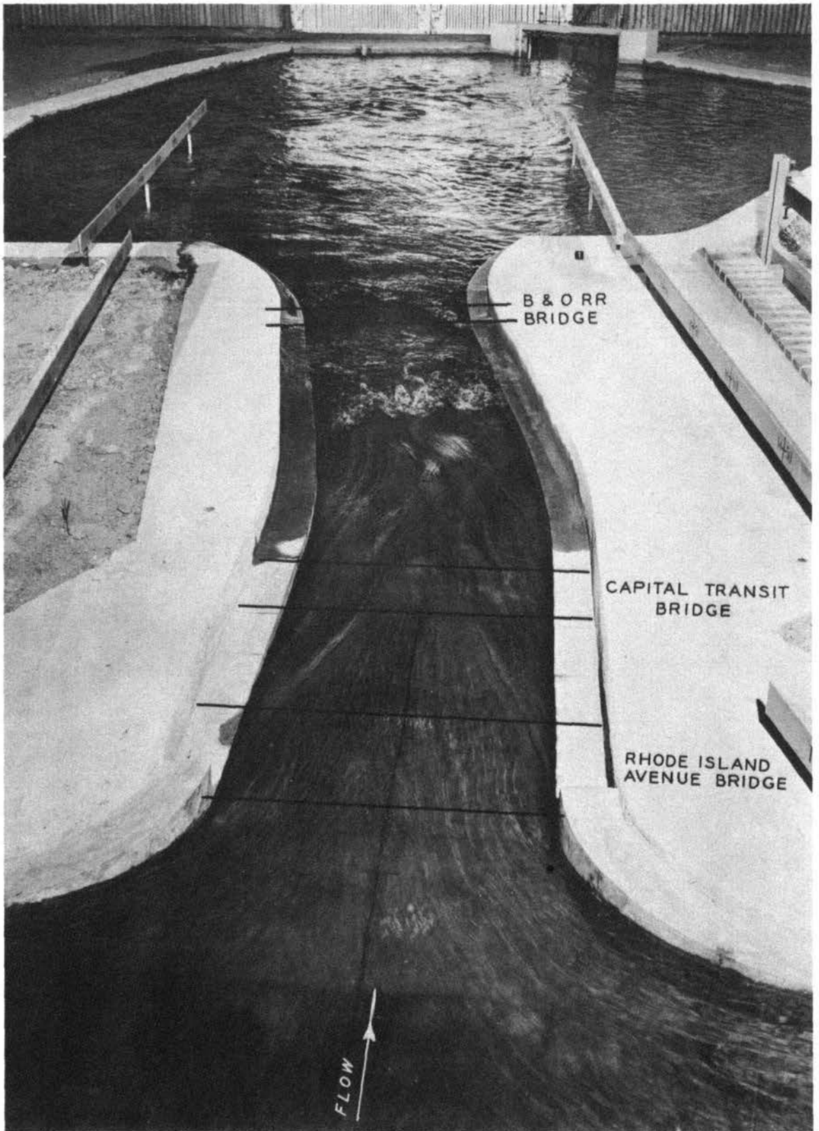
Photograph 5. Original design: flow conditions from upstream end of paved channel to lower end of model. Discharge, 20,000 cfs; tail-water elevation, 19.4 ft msl
