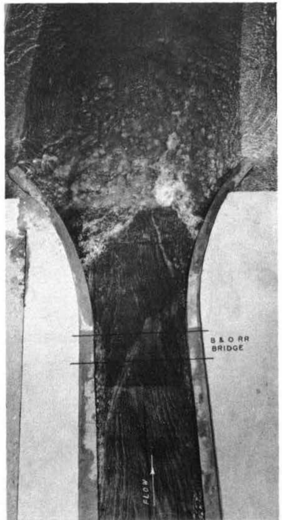
Photograph 3. Original design: position of hydraulic jump extending below the end of paved channel. Discharge, 20,000 cfs; tailwater elevation, 13.5 ft msl
