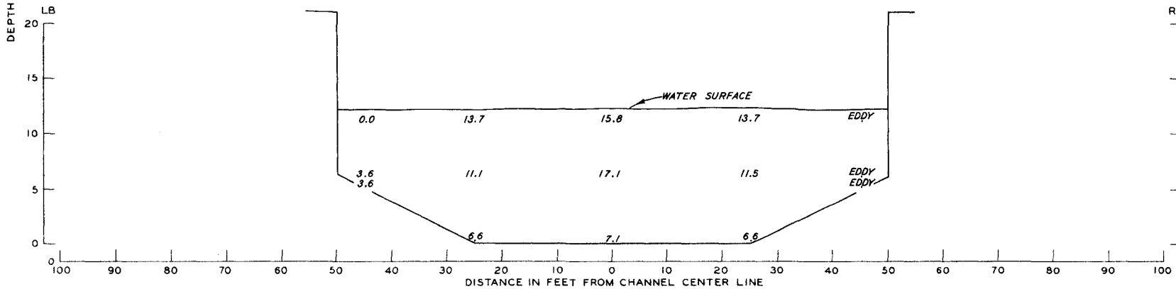
STATION 11+70
