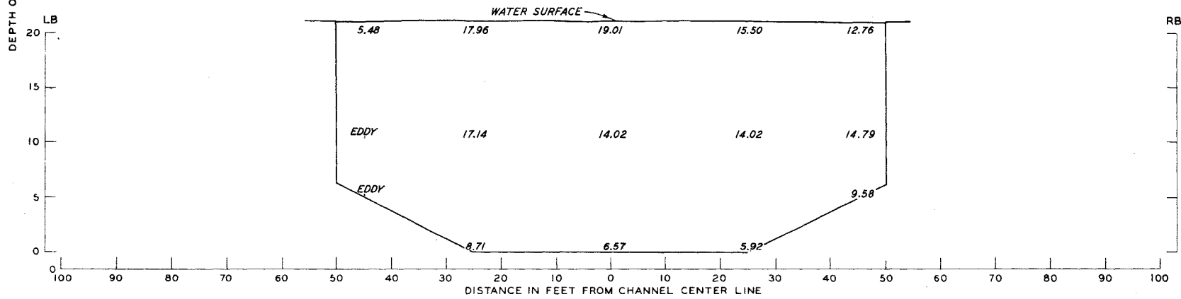
STATION 11+70
