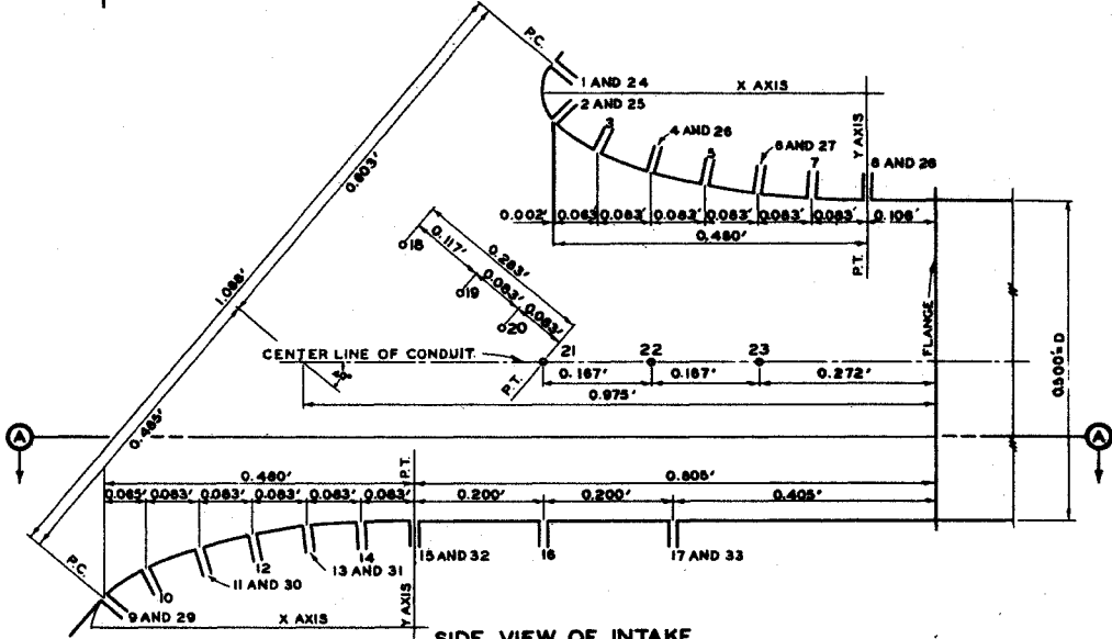
SIDE VIEW OF INTAKE
