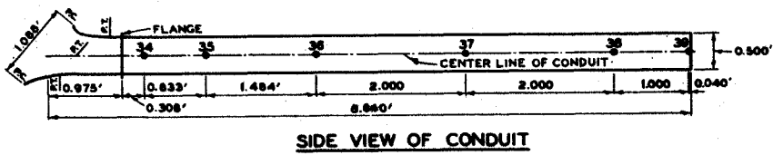
SIDE VIEW OF CONDUIT
