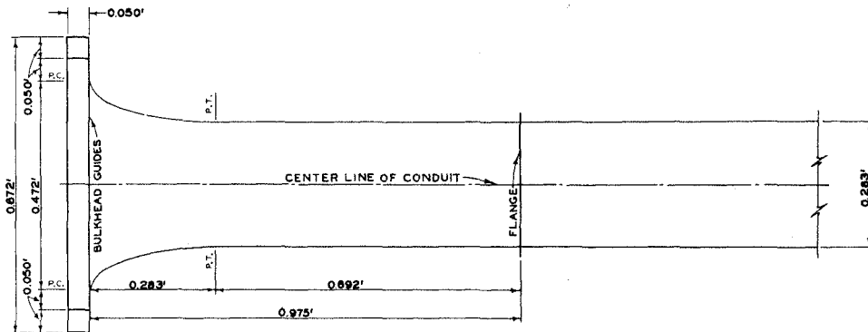
TOP VIEW OF INTAKE
