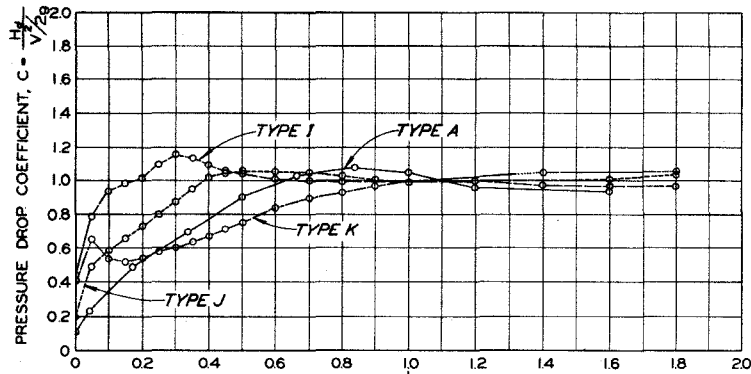
TOP CENTER LINE PIEZOMETERS
