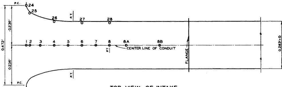
TOP VIEW OF INTAKE
