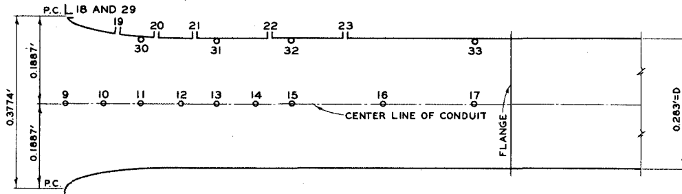
SECTION A
