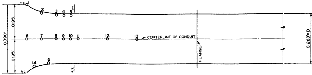
TOP VIEW OF INTAKE
