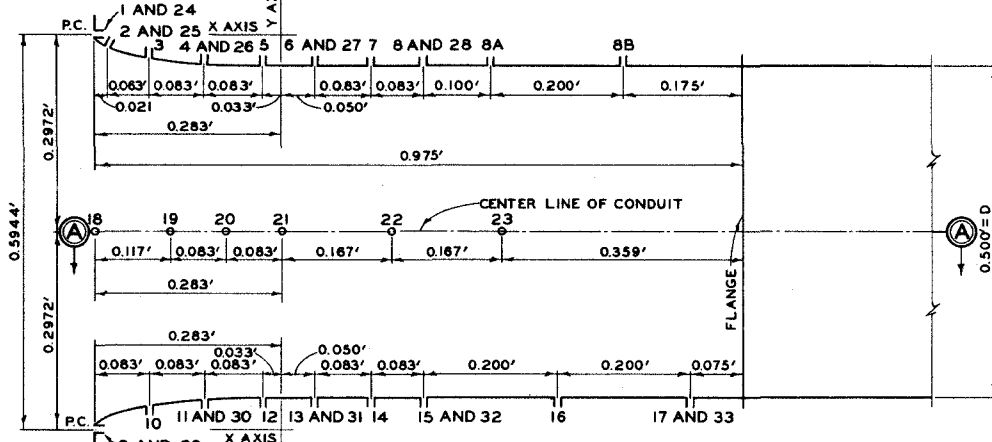
SIDE VIEW OF INTAKE
