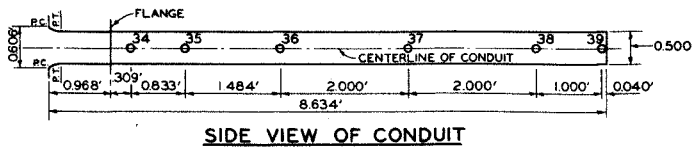
SIDE VIEW OF CONDUIT
