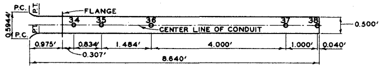
SIDE VIEW OF CONDUIT
