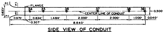
SIDE VIEW OF CONDUIT
