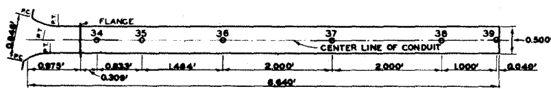
SIDE VIEW OF CONDUIT
