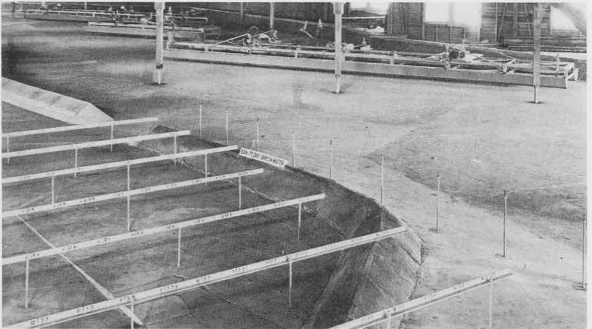
Fig. 4. Wave machines
