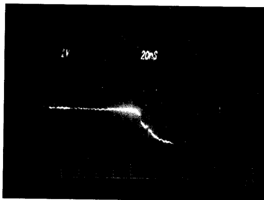
Figure 7 Oscilloscope trace showing the output of a photo-multiplier tube indicating switch closure.
