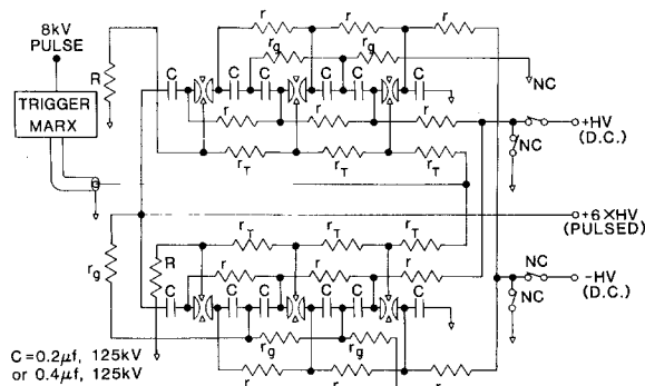
Figure 9 HDZP Marx module circuit diagram.
