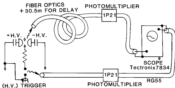
Figure 6 Schematic for jitter tests.
