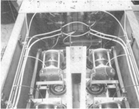
Figure 10 Marx module showing connection between Marx unit outputs.
