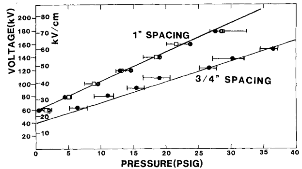
Figure 5 Static breakdown curve for 2.54 cm (1") and 1.9 cm (3/4") electrode spacing.
