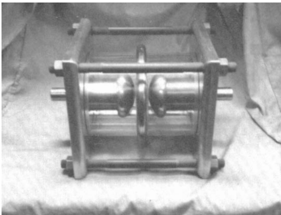
Figure 3 200 kV field distortion switch.
