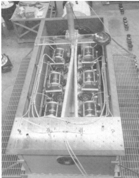
Figure 11 Marx module with trigger Marx unit. 3
