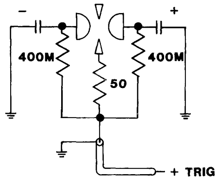
Figure 4 Static breakdown test circuit.
