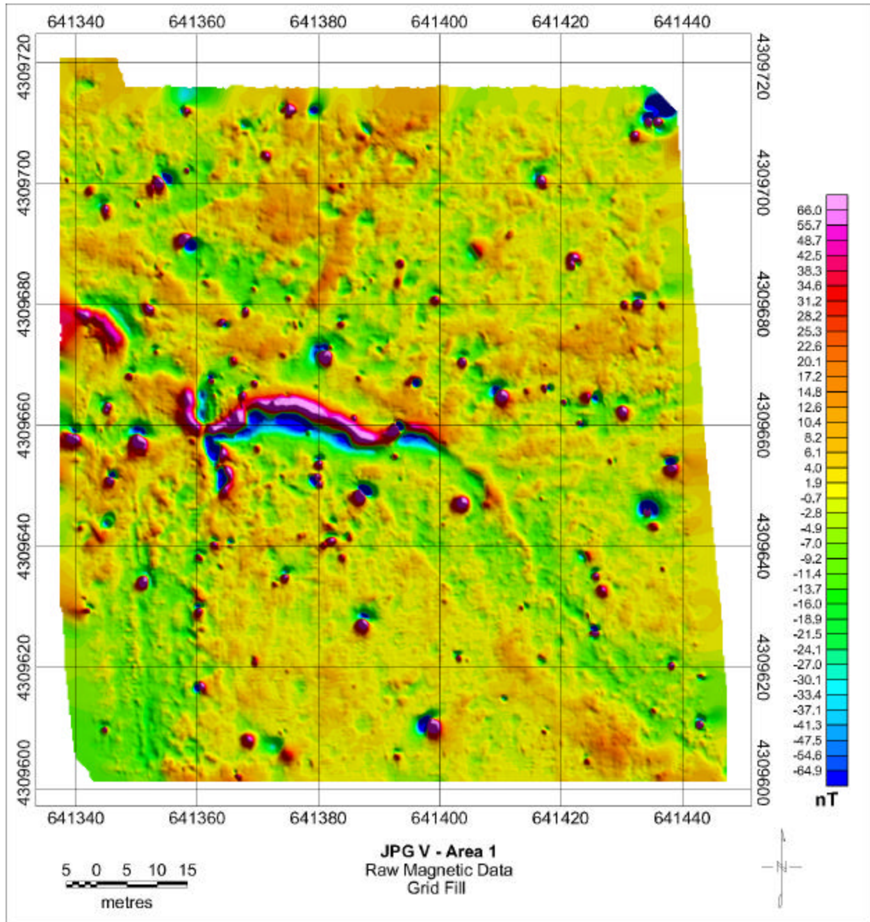
Figure 8. Color-coded map of the MTADS magnetic data, Area 1 JGP TD. Note that the data gaps apparent in Figures 6 and 7 have been interpolated.
