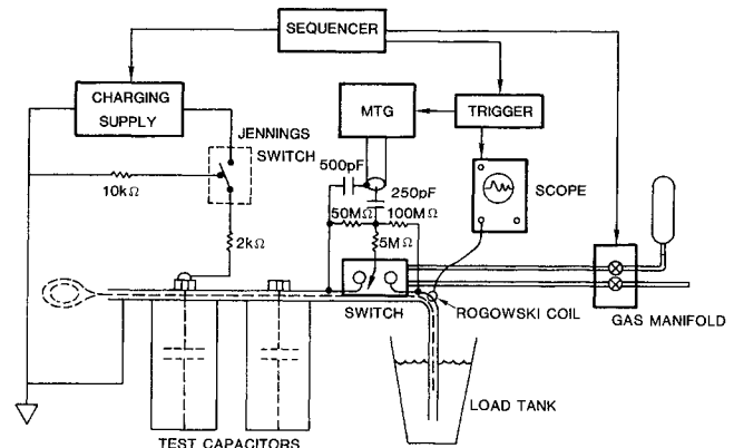
Figure 1. Capacitor life test arrangement.
