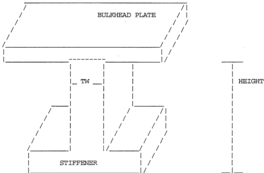
FIGURE 7 - Stiffener characteristics
