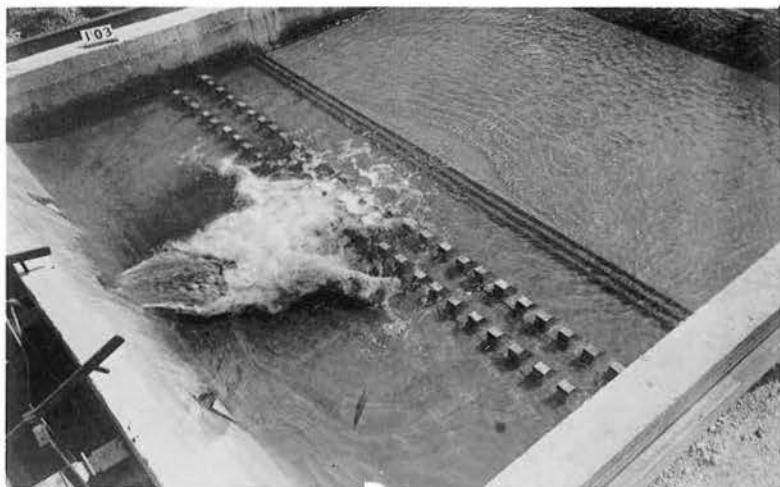
a. Discharge 1640 cfs Pool elev 948.5 Tailwater elev 911.6
