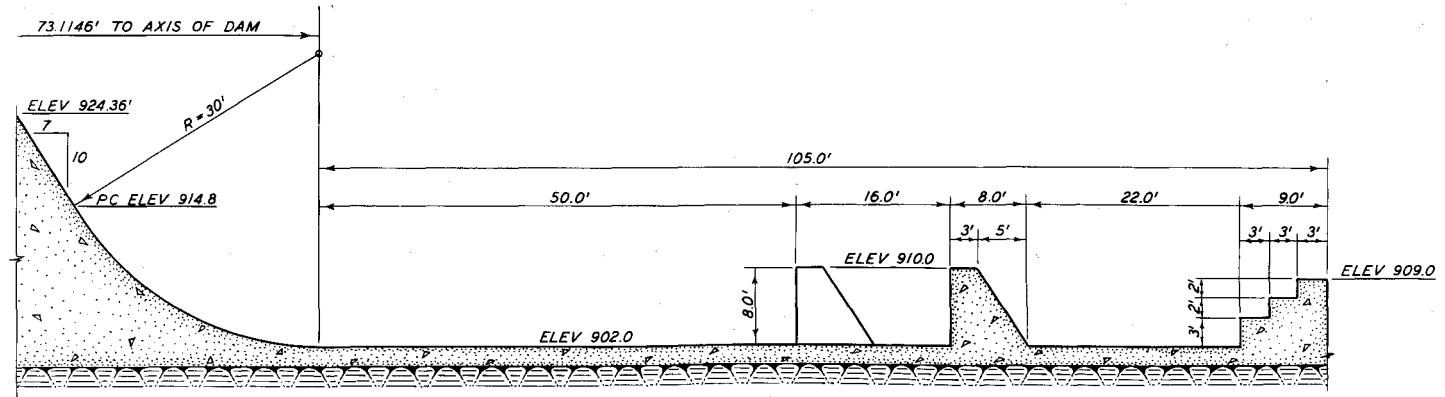
TYPE 2 BASIN
