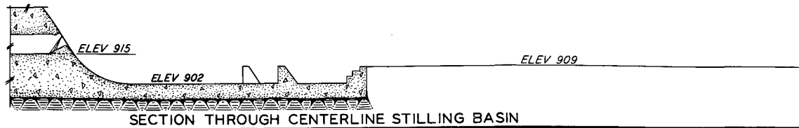
SECTION THROUGH CENTERLINE STILLING BASIN
