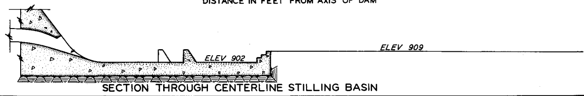
MODEL STUDY OF SLUICES FALL RIVER DAM FALL RIVER, KANSAS SCOUR PATTERN
