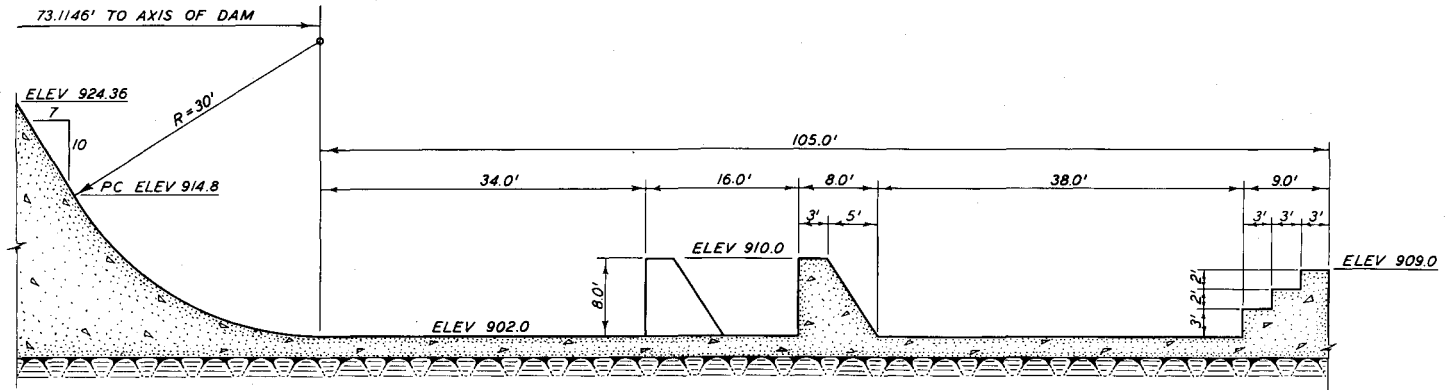
TYPE 1 BASIN
