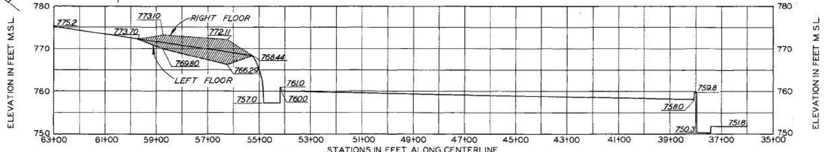
FLOOR ELEVATIONS ALONG MAIN CHANNEL
