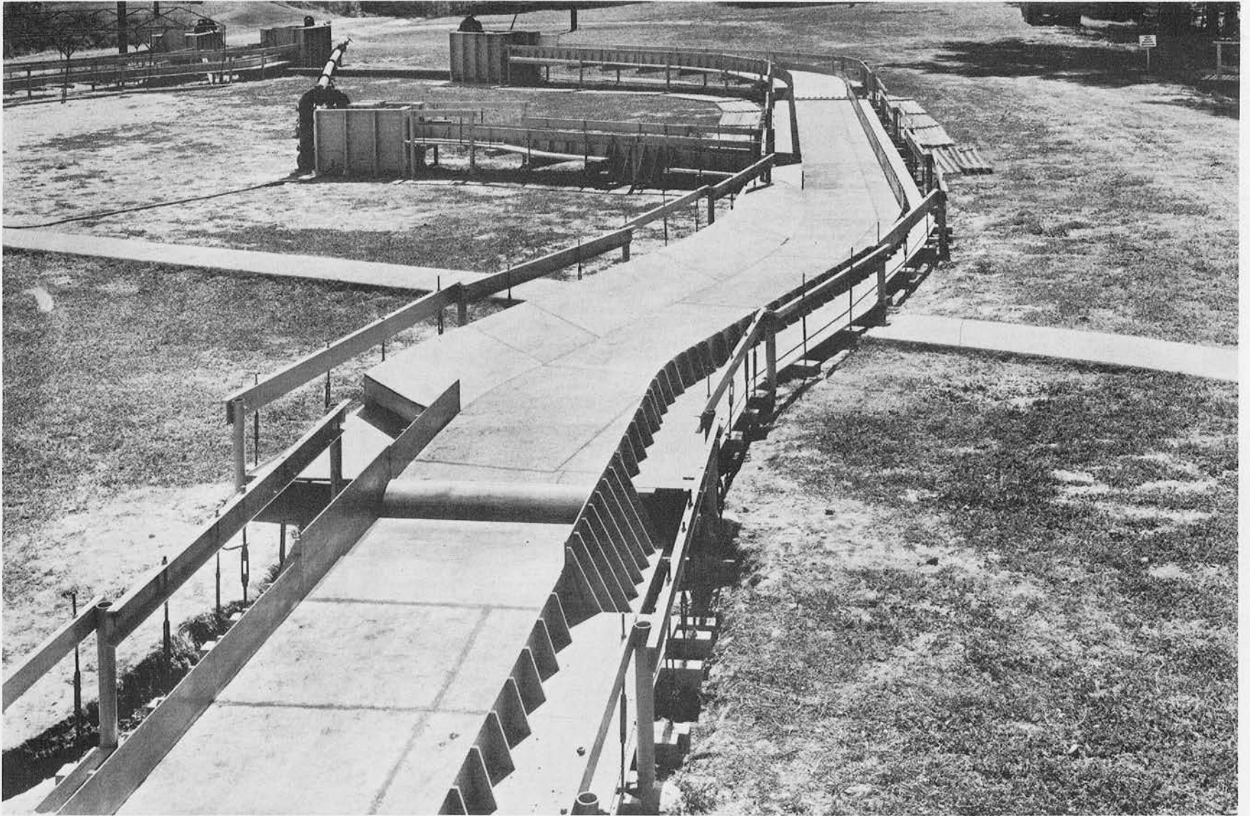
Upstream view, Adams model. Hoosic River, original design
