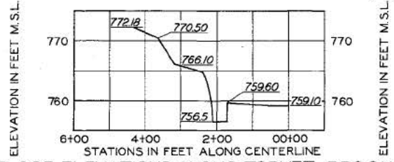
FLOOR ELEVATIONS ALONG TOPHET BROOK
