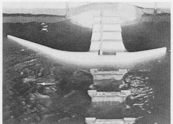
Fig. 8. Free flow Type 1 weir, type C abutment wall, discharge 490,000 cfs
