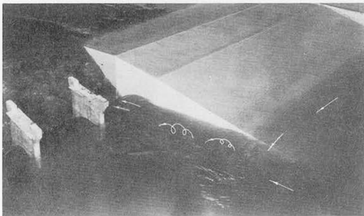
Fig. 4. Pool elev 53.6; minimum tailwater Discharge 490,000 cfs
