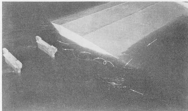
Fig. 5. Pool elev 56.9; tailwater elev 55.7 Discharge 490,000 cfs
