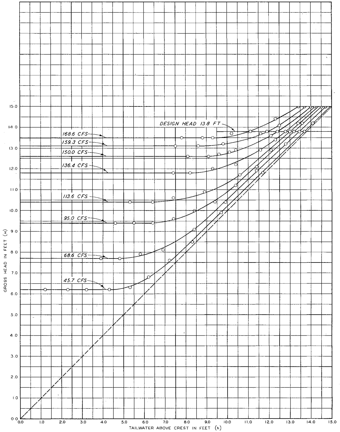
MODEL SCALE 1:30 SUBMERGENCE CURVES TYPE 2 WEIR
