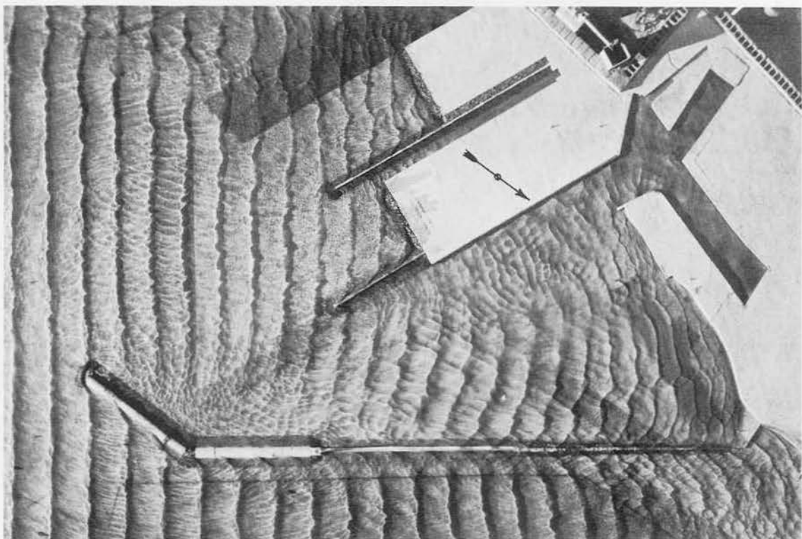
Figure 18. Plan Y with 6.5-sec waves 15.5-ft high from south-southeast
