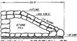
TYPICAL SECTION OF WAVE ABSORBER
