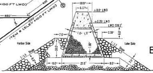
SECTION A TYPE BREAKWATER
