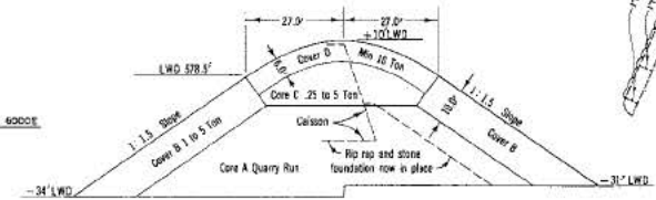
SECTION D TYPE BREAKWATER
