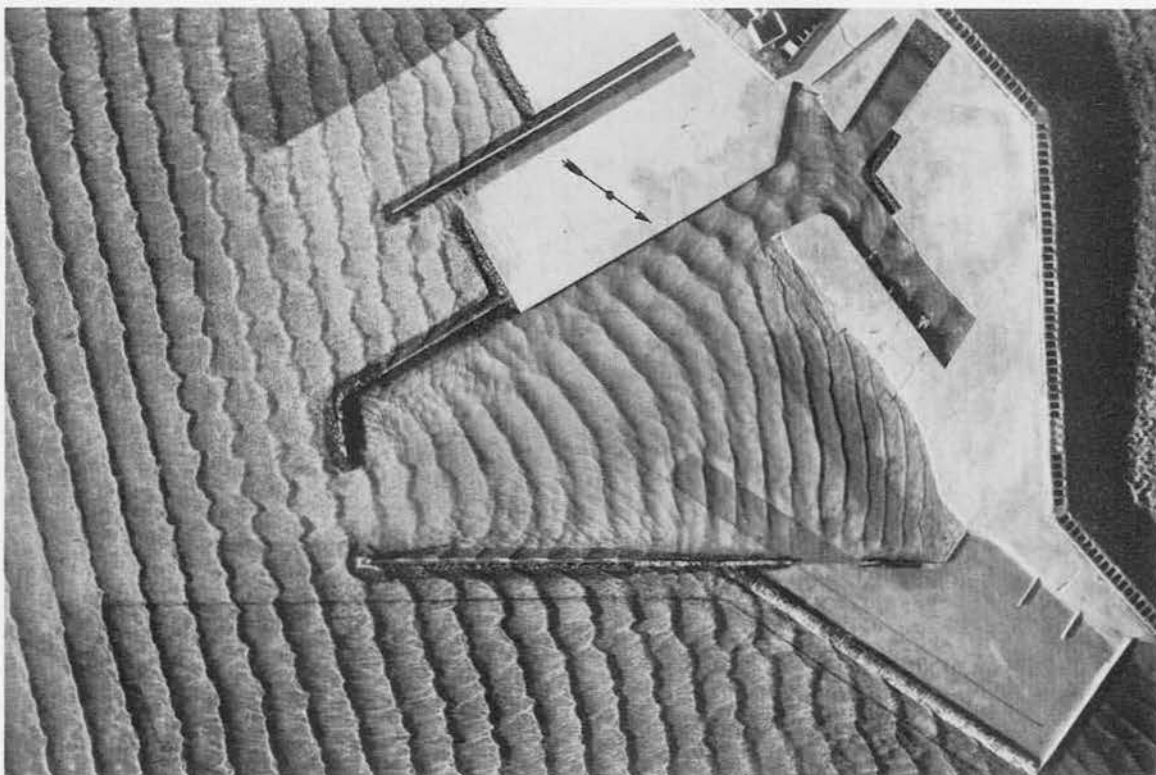
Figure 6. Plan E-1 with 6.0-sec waves 14.5-ft high from the southeast
