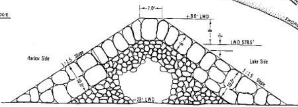
SECTION C TYPE BREAKWATER
