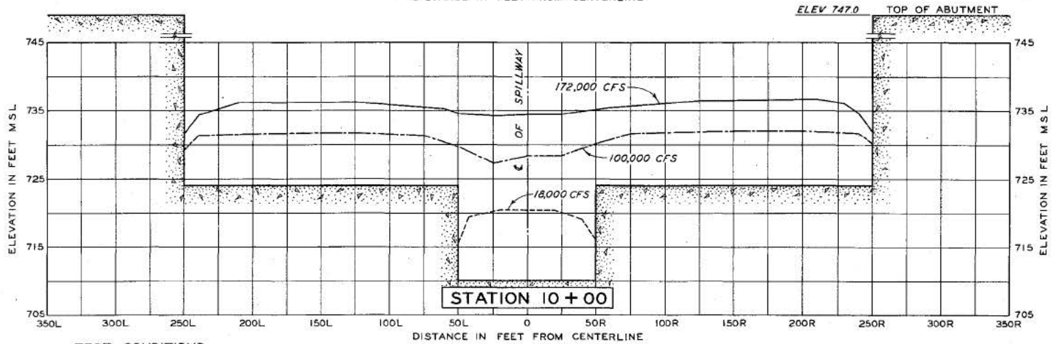
WATER-SURFACE CROSS SECTION AT SPILLWAY CREST
