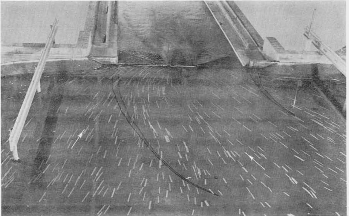
a. Discharge 18,000 cfs; pool elevation 724.0 ft
