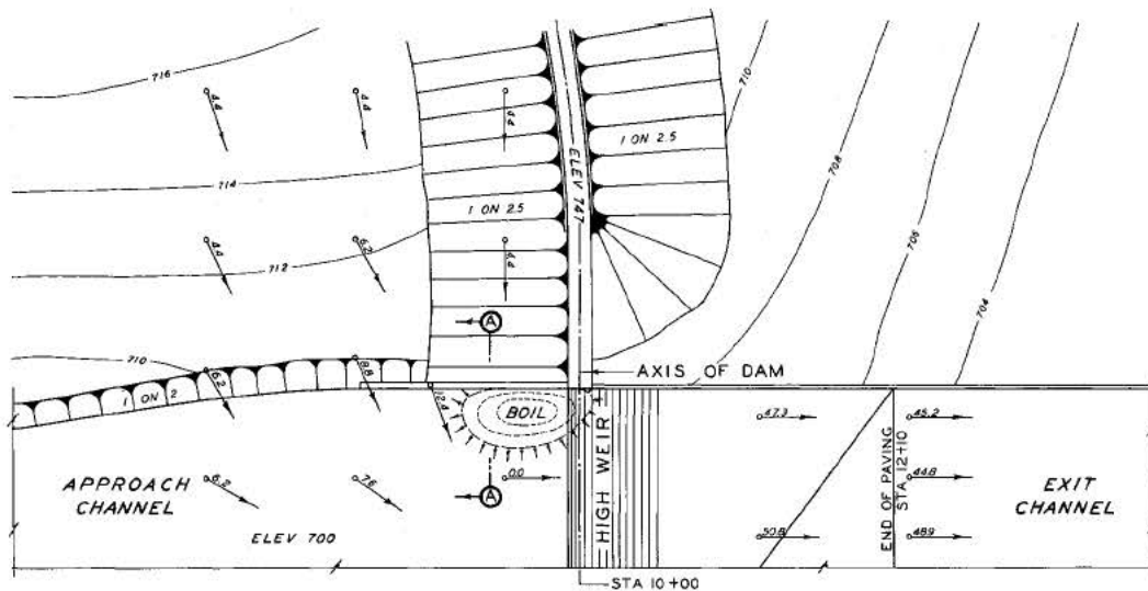
2ND ALTERNATE - 3 FT PARAPET
