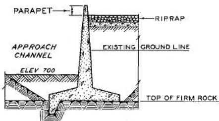
SECTION A-A (SCHEMATIC)
