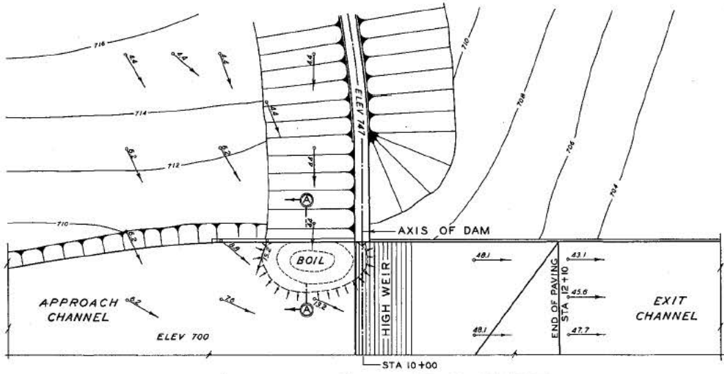
4TH ALTERNATE - 7 FT PARAPET
