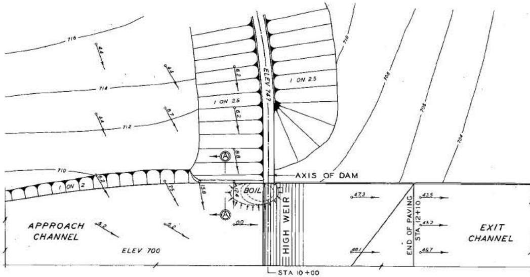
1ST ALTERNATE - NO PARAPET
