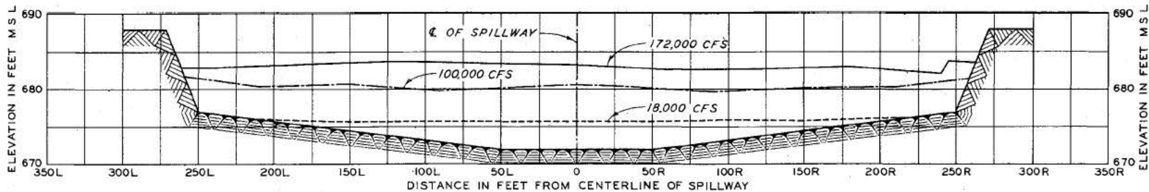
STATION 23 + 00
