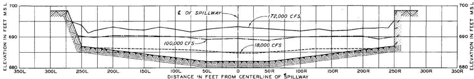
STATION 16 + 00
