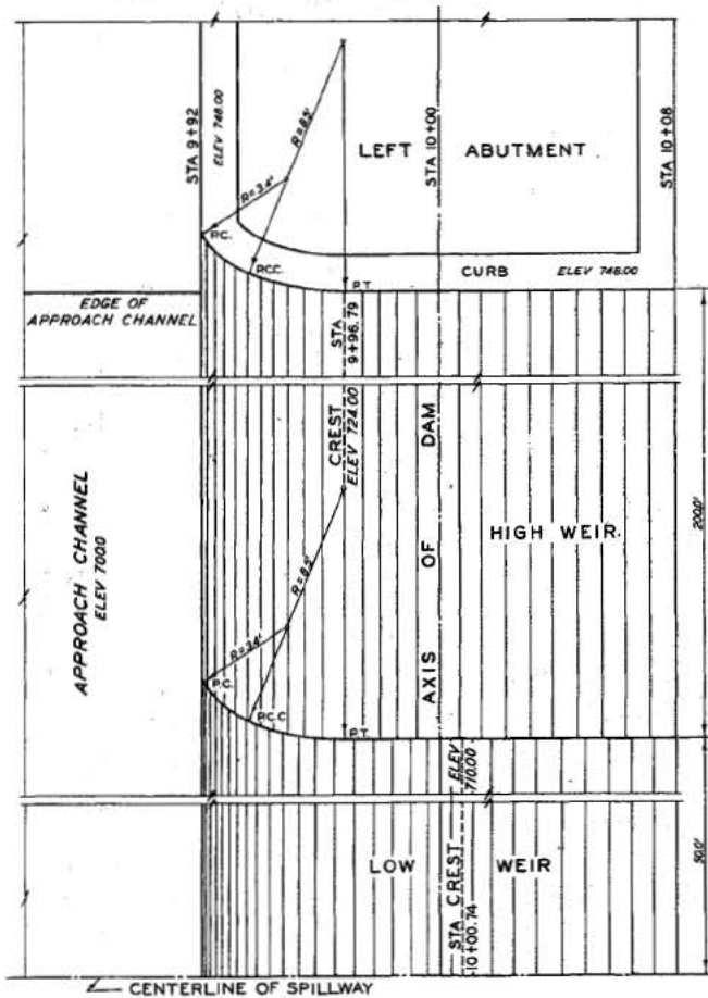
HALF PLAN
