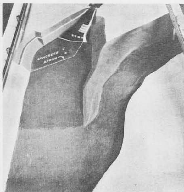
Fig. 17. Recommended stilling-basin design with left training wall terminated at end sill
