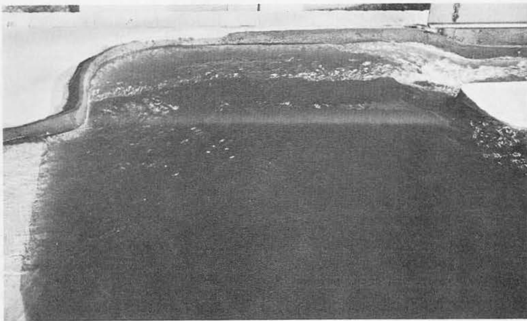
HEAD = 24.4 FT DISCHARGE = 93,500 CFS
