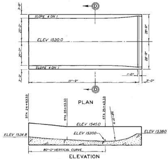
TYPE AI DESIGN
