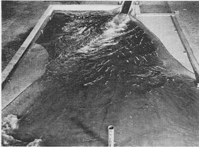
Fig. 5. Type B bucket flow characteristics Discharge, 70,000 cfs; tailwater, 1549.9 Observation of bucket action during various discharges disclosed that flow was too concentrated and indicated that scour immediately downstream from the bucket would be excessive. Fig. 5 shows flow characteristics of this design for the maximum discharge. No other tests were made on this bucket.
