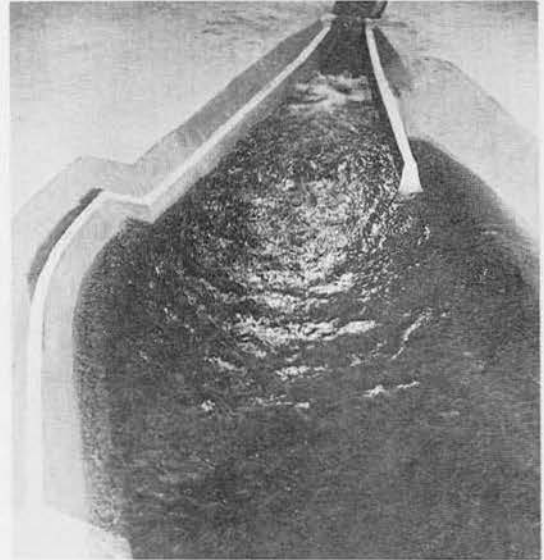
Discharge, 2,500 cfs; tailwater, 1528.5
