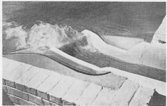
Discharge, 10,000 cfs; falling pool stage
