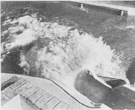
DISPERSAL BUCKET
