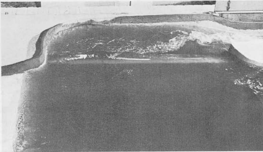
HEAD = 20.1 FT DISCHARGE = 82,320 CFS
