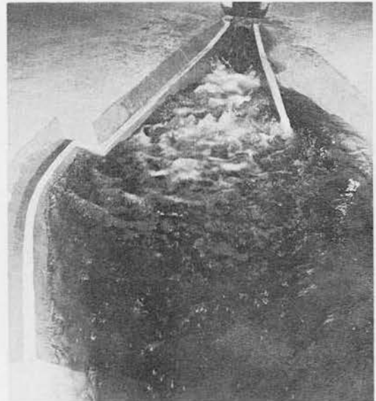
Discharge, 5,000 cfs; tailwater, 1531.0
