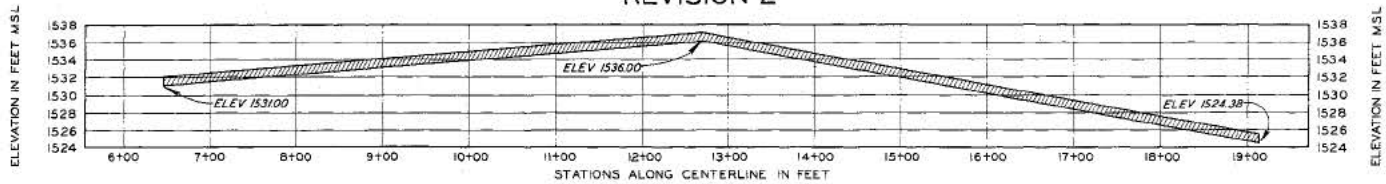
REVISIONS OF GRADE OUTLET WORKS CONDUIT
