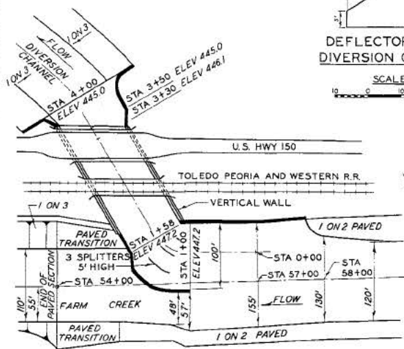
PLAN 3
