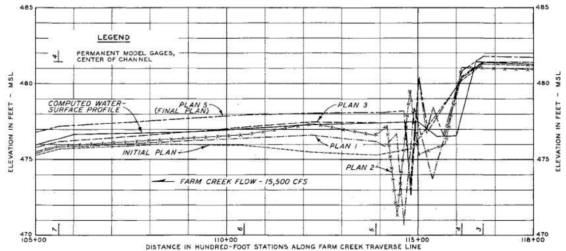
WATER-SURFACE PROFILES - FARM CREEK
