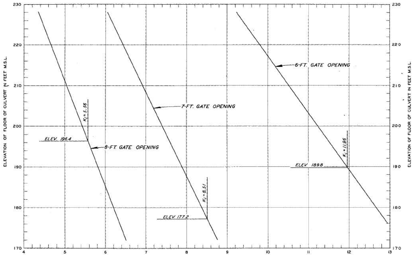
ME NARY DAM, OREGON MODEL OF TAINTER VALVE CAVITATION PARAMETER VERSUS CULVERT INVERT ELEVATION
