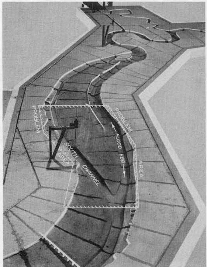
Fig. 3. Upstream view of south channel problem area
