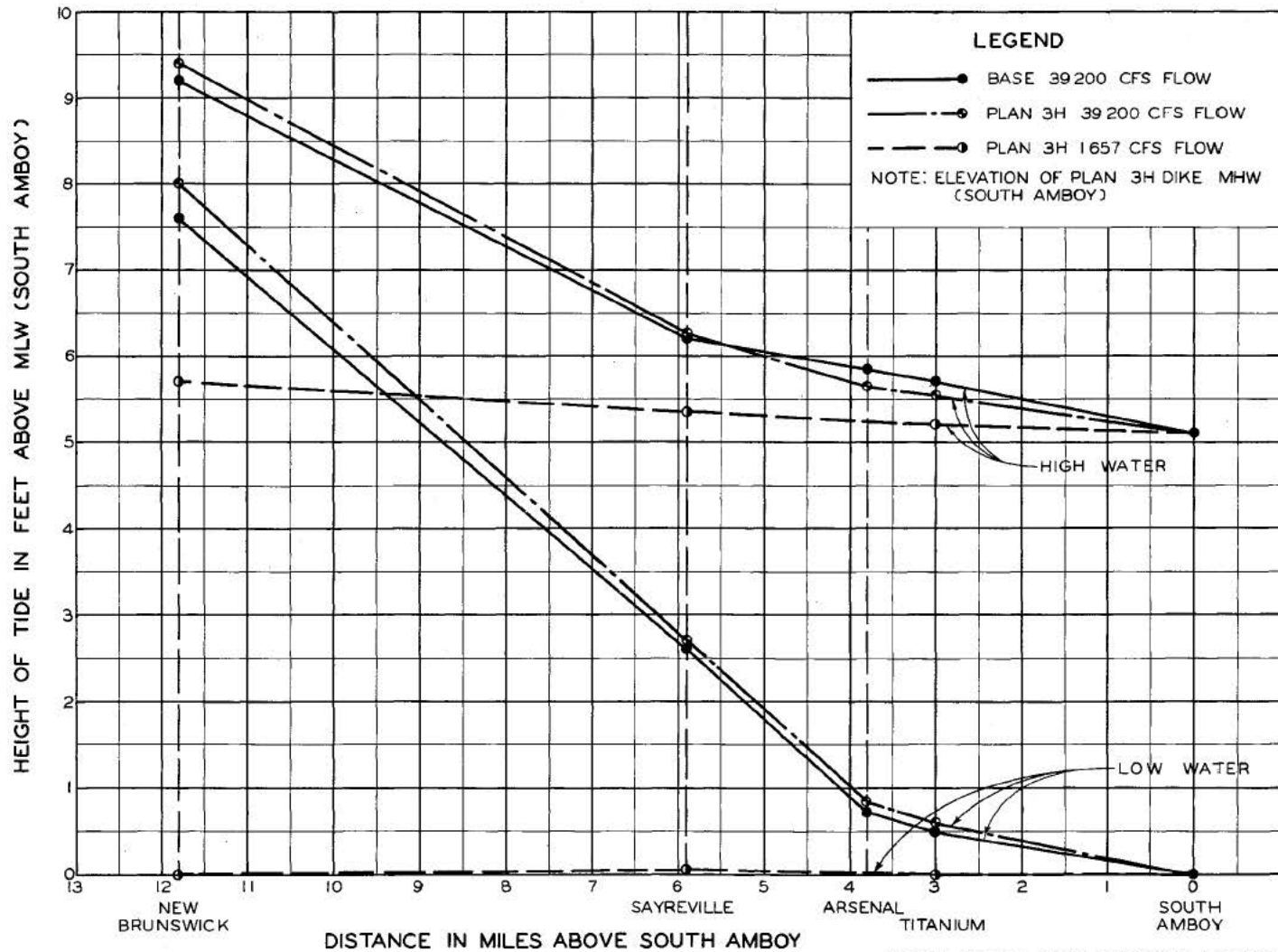
HIGH AND LOW WATER PROFILES PLAN 3H
