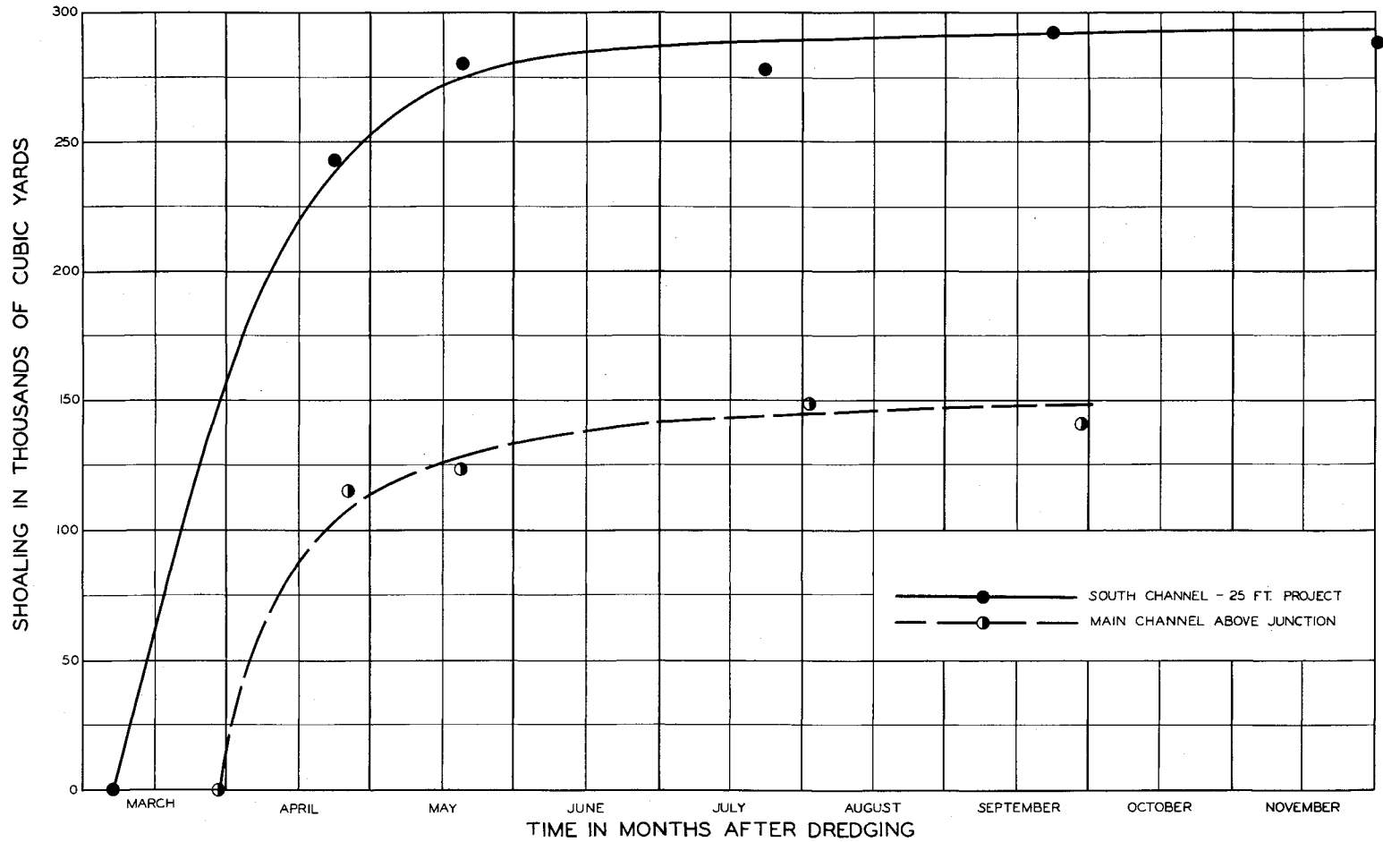
AFTER DREDGING SURVEYS MAIN CHANNEL AND SOUTH CHANNEL 25 FT. PROJECT
