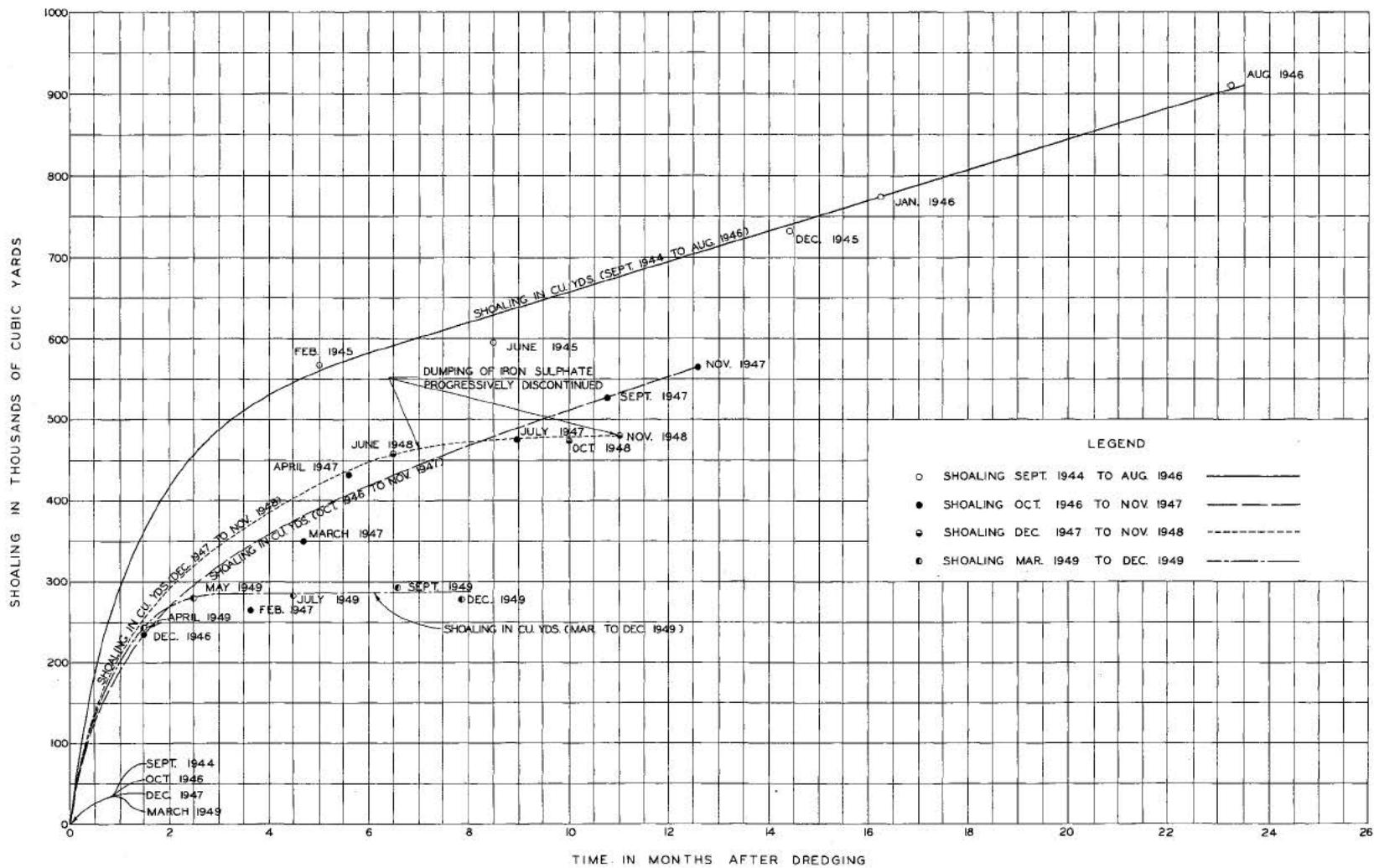
SHOALING - SOUTH CHANNEL 25 - FOOT PROJECT
