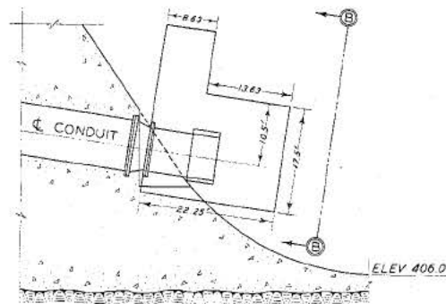
SECTION THROUGH CENTERLINE OF CONDUIT TYPE 2 HOOD
