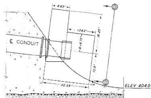
SECTION THROUGH CENTERLINE OF CONDUIT TYPE 4 HOOD
