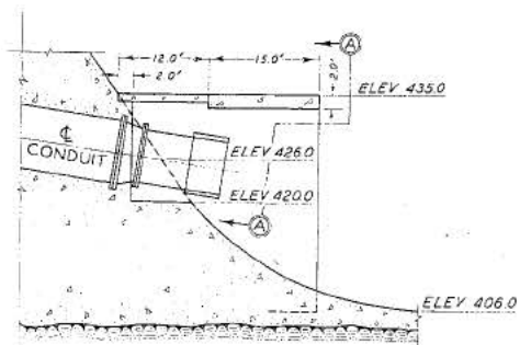
SECTION THROUGH CENTERLINE OF CONDUIT TYPE 1 HOOD
