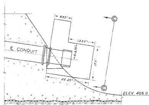
SECTION THROUGH CENTERLINE OF CONDUIT TYPE 3 HOOD
