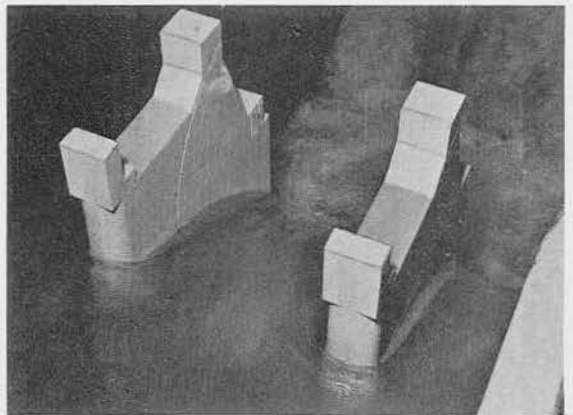
Discharge 250,000 cfs
