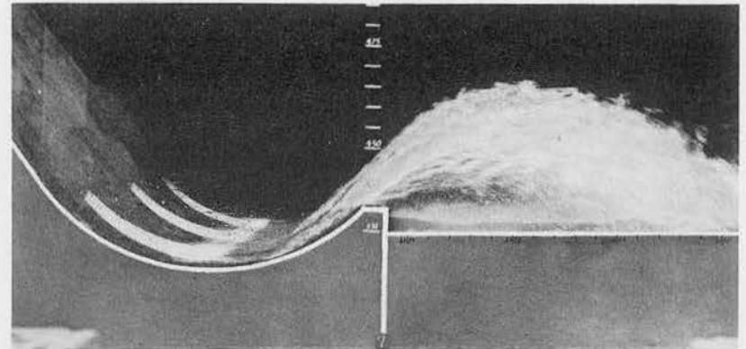
8 conduits Discharge 20,000 cfs; tailwater elev 438.4 Pool elev 528.95
