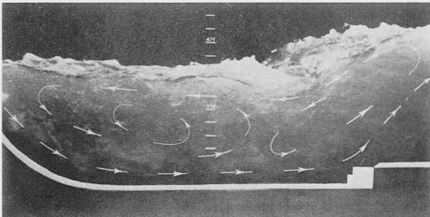
6-ft end sill, no baffles Discharge 250,000 cfs; TW elev 475.4; pool elev 555.03
