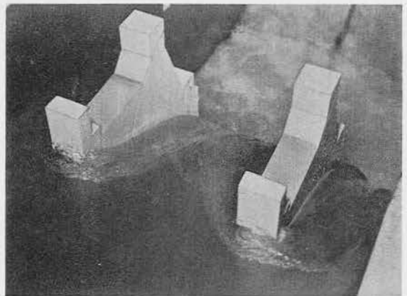
Discharge 660,000 cfs
