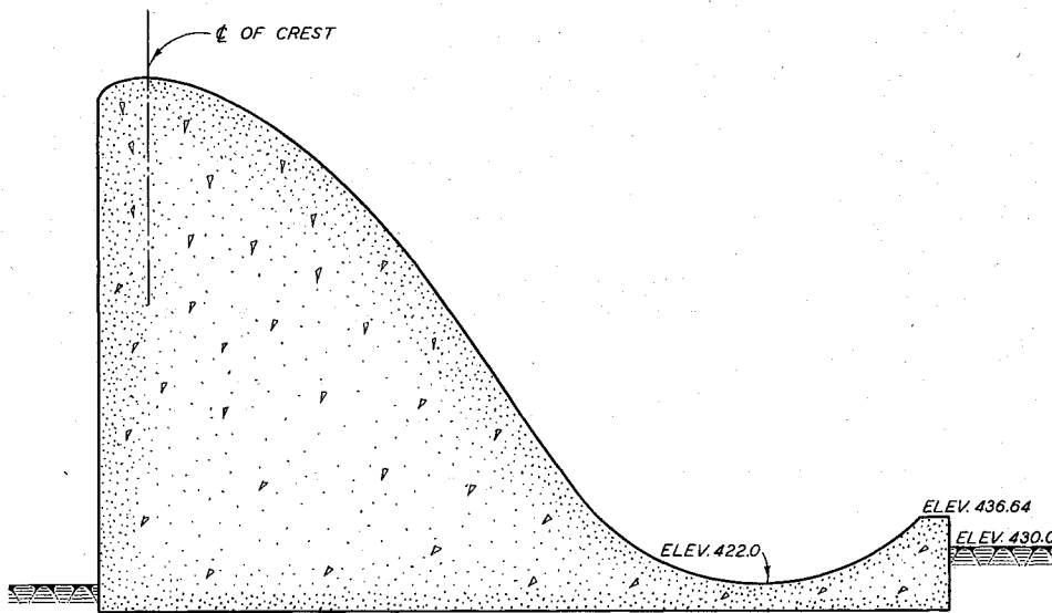
TYPE I BUCKET - ORIGINAL DESIGN
