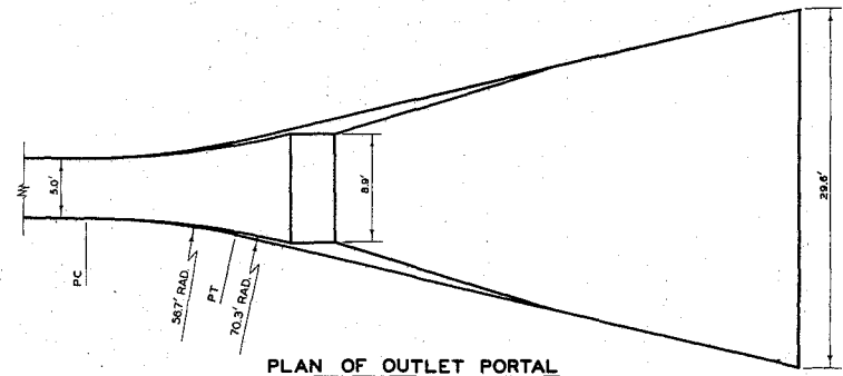
PLAN OF OUTLET PORTAL
