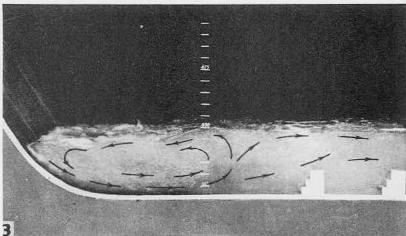
Discharge 50,000 cfs; TW elev 448.3; pool elev 540.86
