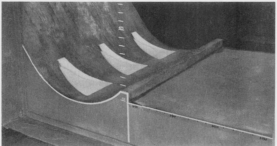
Fig. 3. Type 1 bucket
