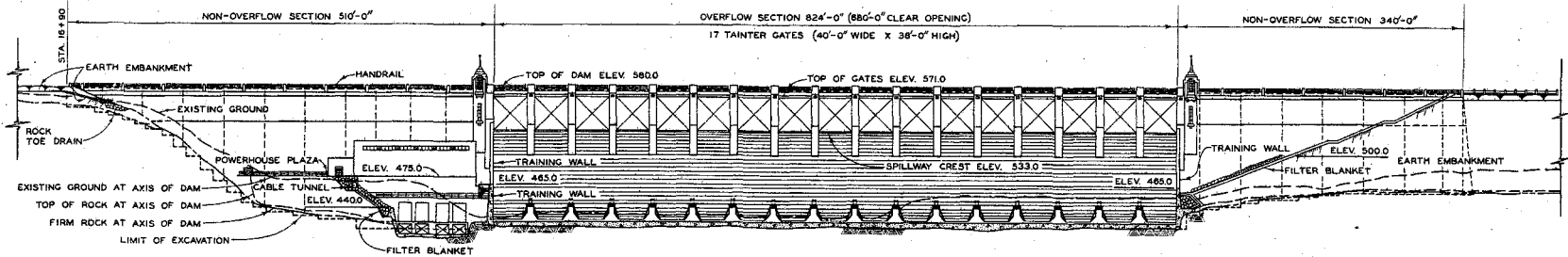
DOWNSTREAM ELEVATION
