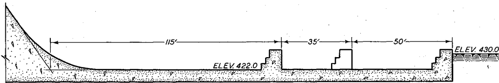
TYPE I APRON - ORIGINAL DESIGN
