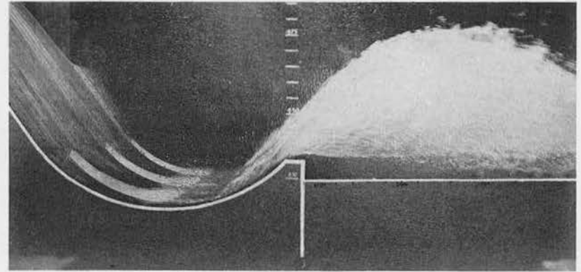
12 conduits Discharge 36,000 cfs; tailwater elev 444.4 Pool elev 570.50
