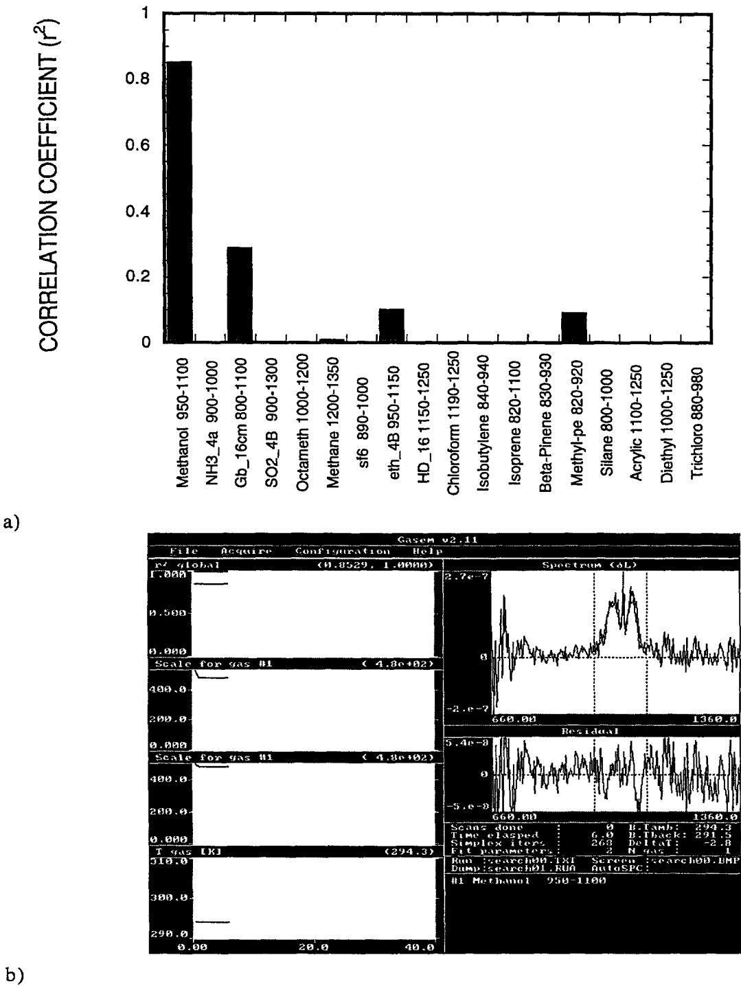
FIGURE 13 -Example of the search functionality for methanol: (a) the correlation factors obtained for each of the 18 hypothetical chemicals and (b) the resulting spectral match for the highest r^2 scored with methanol.
