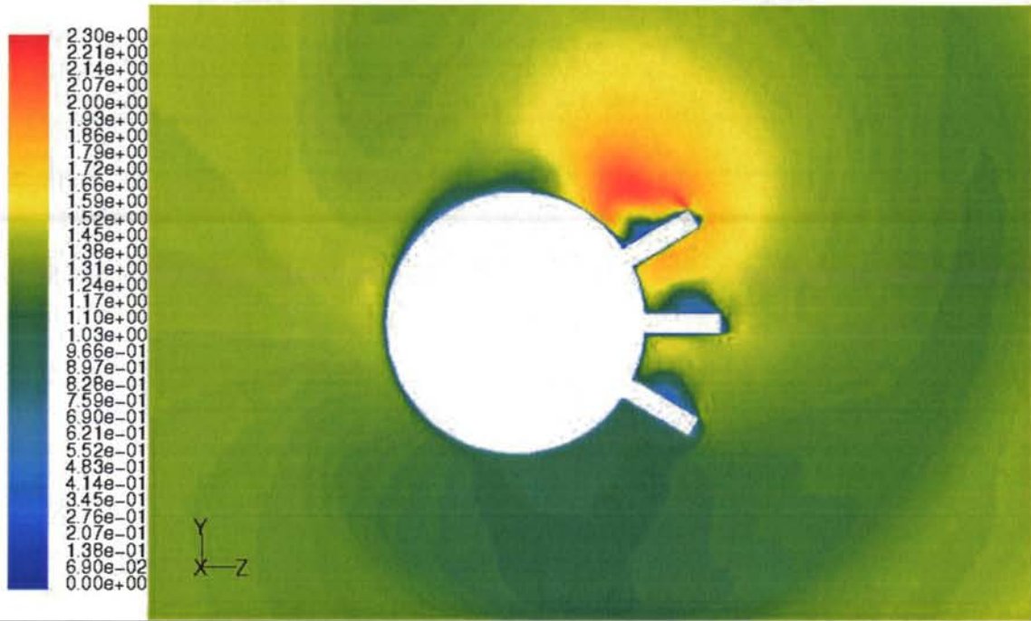
Contours of Mach Number Mar 25, 2004 FLUENT 6.1 (3d, coupled exp, rke)
