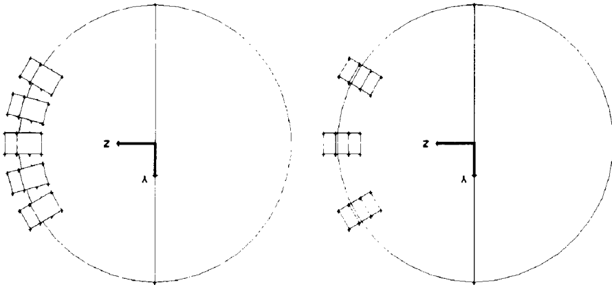
Figure 4: Position of the baseline FE on the aerodynamic geometry
