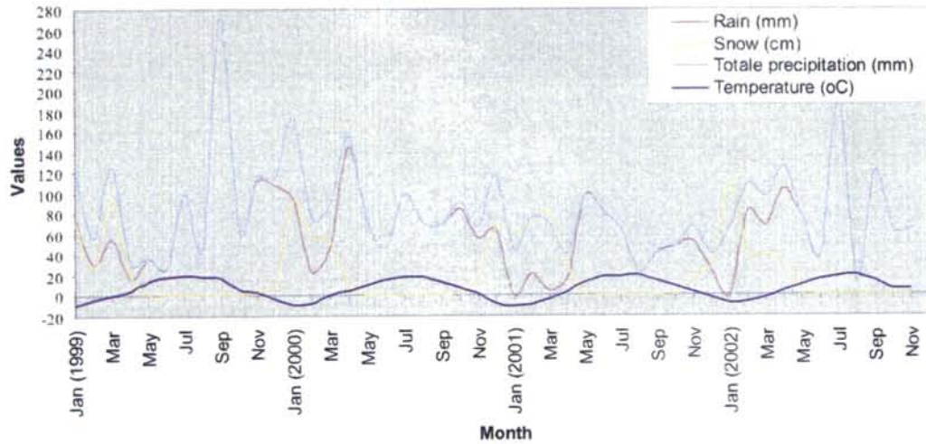
Figure 1. Fluctuations of meteorological data at Fredericton weather station (1999-2002)
