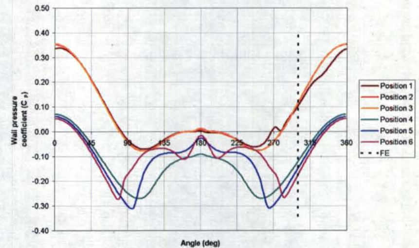
Figure C19 : Wall pressure profiles with KFE at 300° and 15° AOA
