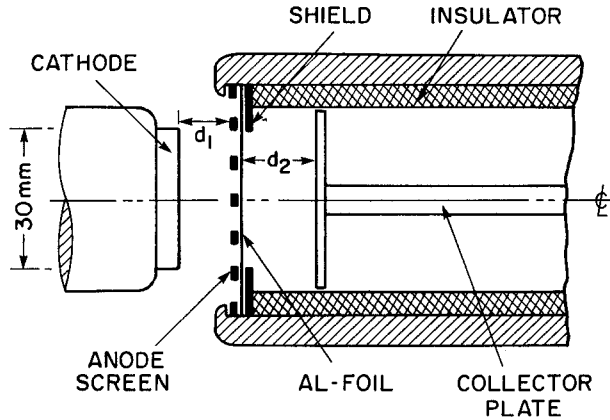
Figure 3. Schematic of the electrode and collector structure of the two-pulse diode.
