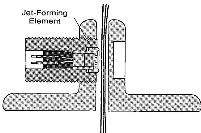
Figure 3 - Improved switch design using a jet-forming element. The switch is shown expanded for clarity.
