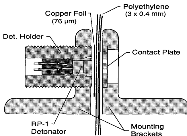
Figure 1 - Expanded view of the explosively actuated closing switch used on Pegasus I. During operation, the dielectric is tightly sandwiched between the detonator and the contact plate.
