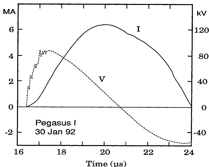
Figure 2 - Current and voltage waveform from Pegasus I, showing the effect of non-ideal switch behavior at early time.
