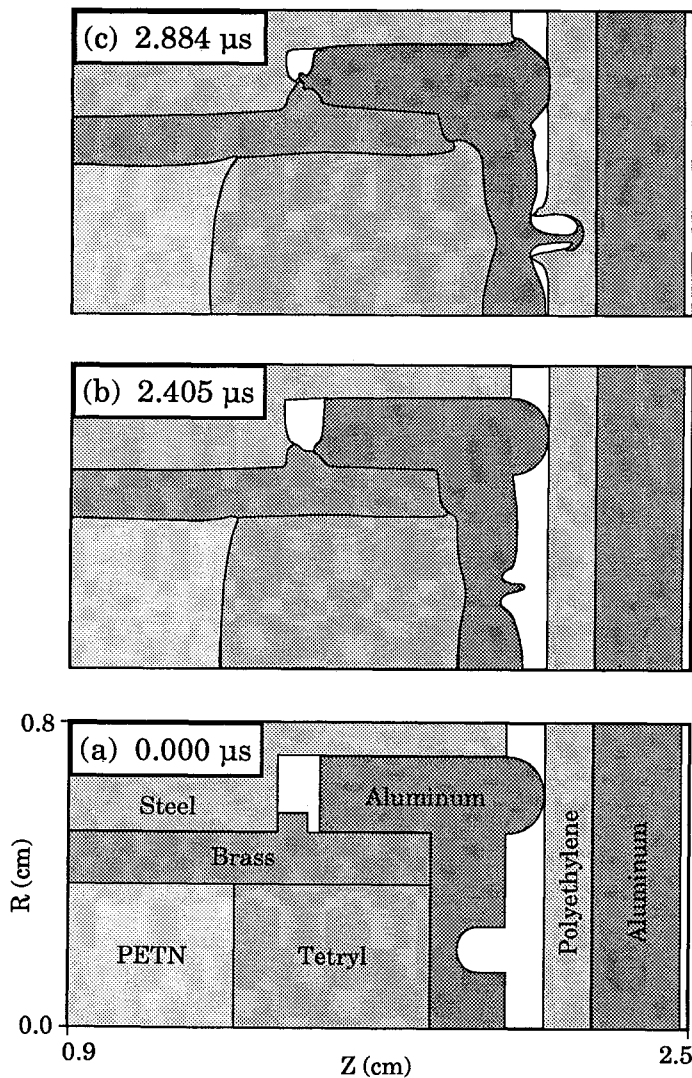
Figure 4 - Predictions of jet motion from the 2-D hydrodynamics calculations. a) initial configuration, b) as the jet begins to form, c) shortly before switch closure.
