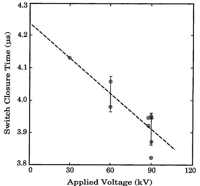
Figure 5 - Measurements of switch closure time vs applied voltage. The dashed line shows the best fit to a simple model of switch delay assuming breakdown at a fixed electric field in the switch dielectric.
