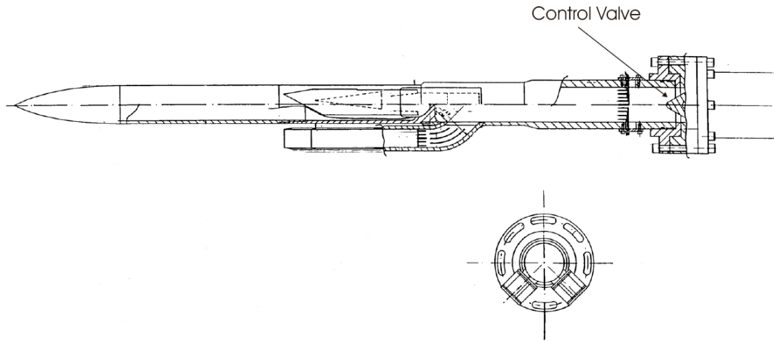
Figure 2: Test configuration used by VOLVO.
