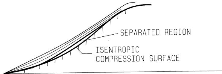
Figure 18: Boundary layer bridging across an isentropic ramp.
