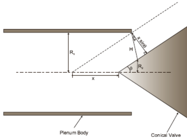
Figure 14: Nomenclature for the cell exit.
