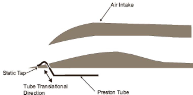
Figure 19: Boundary layer probe traverse set-up.
