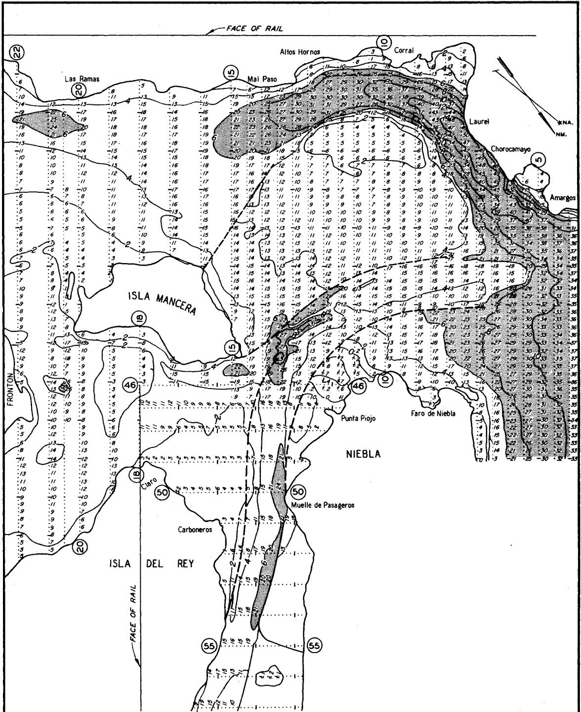
PLAN 4 CONDITION OF MOVABLE BED AT END OF TEST DURATION OF TEST 12 YEARS
