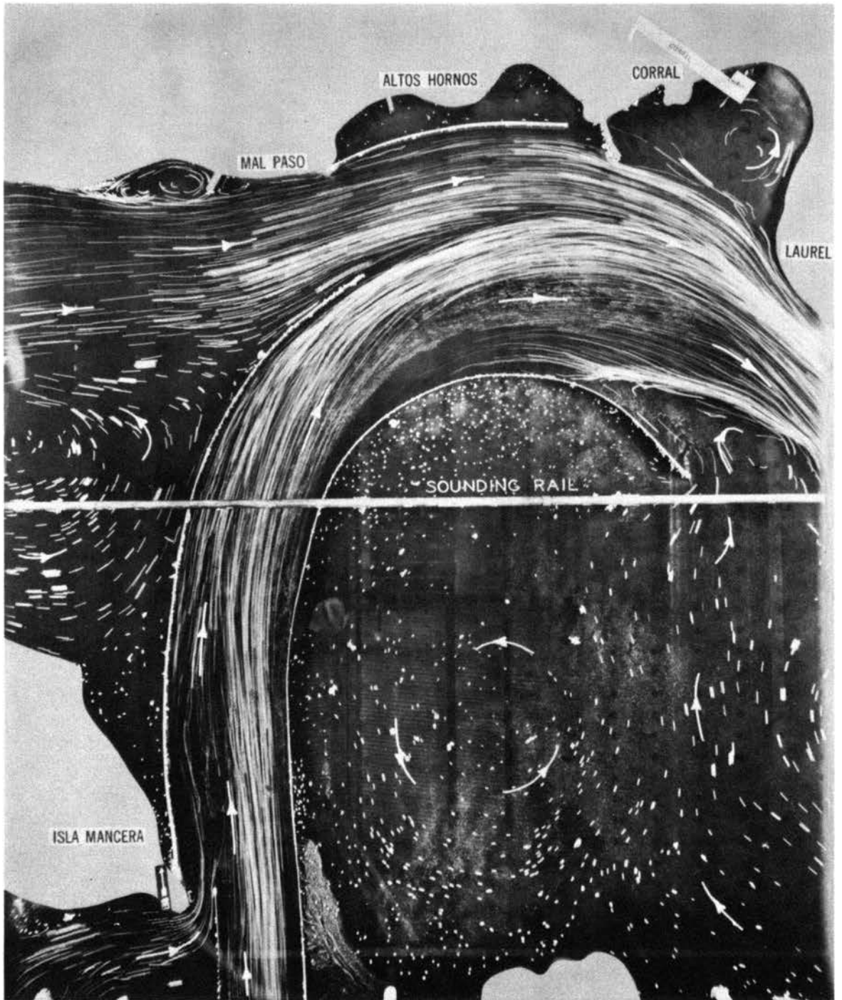
Photograph 6. Strength of ebb, plan 2
