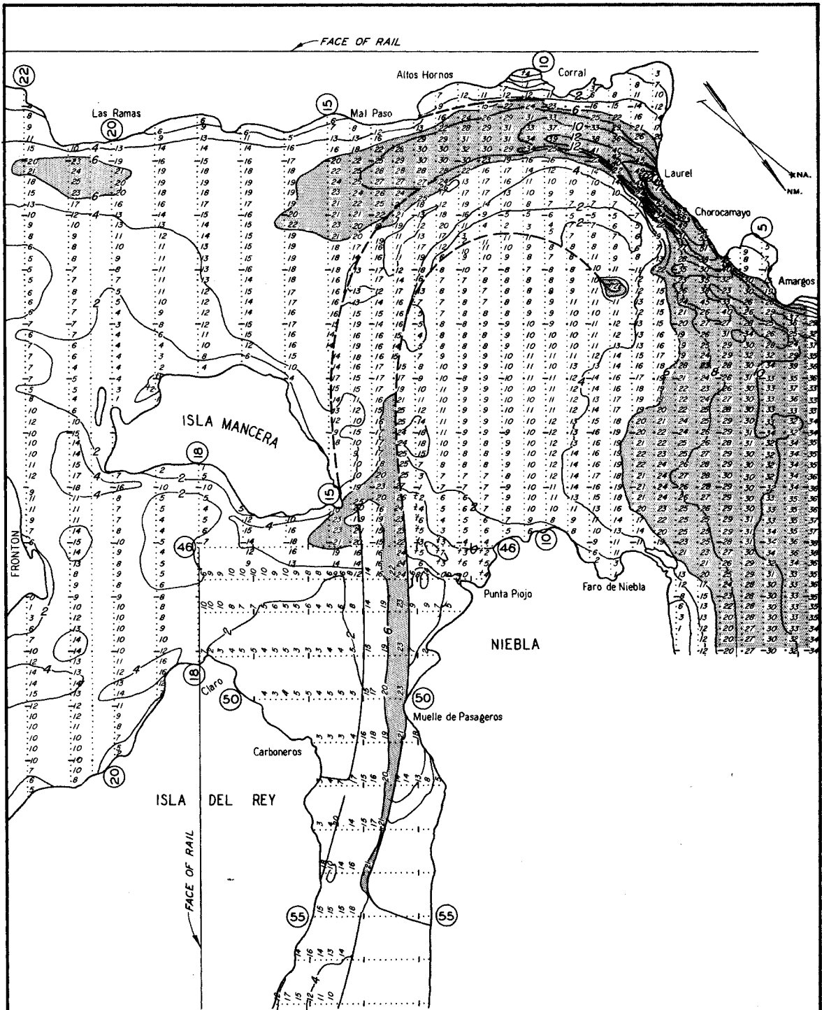
PLAN 2 CONDITION OF MOVABLE BED AT END OF TEST DURATION OF TEST 12 YEARS
