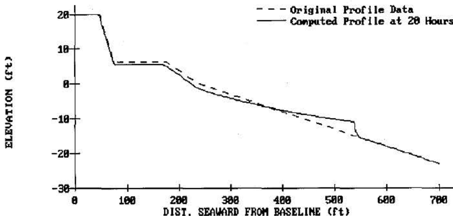
Figure 6-2-4. Profile Change After 20 Hr
