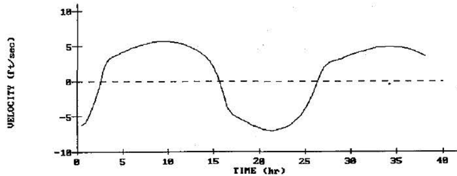
Figure 7-1-10. Velocity Hydrograph at Cell (1,2,2)
