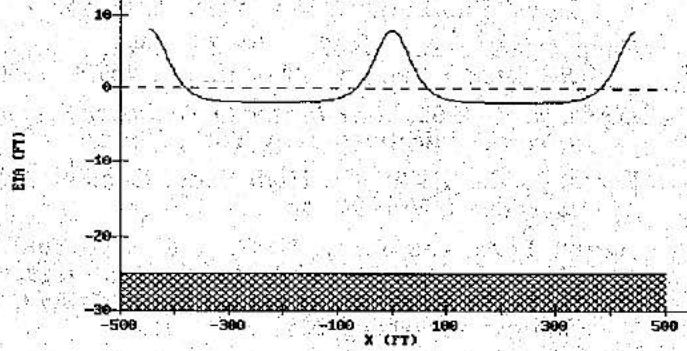
Figure 2-2-7. Water Surface Elevation
