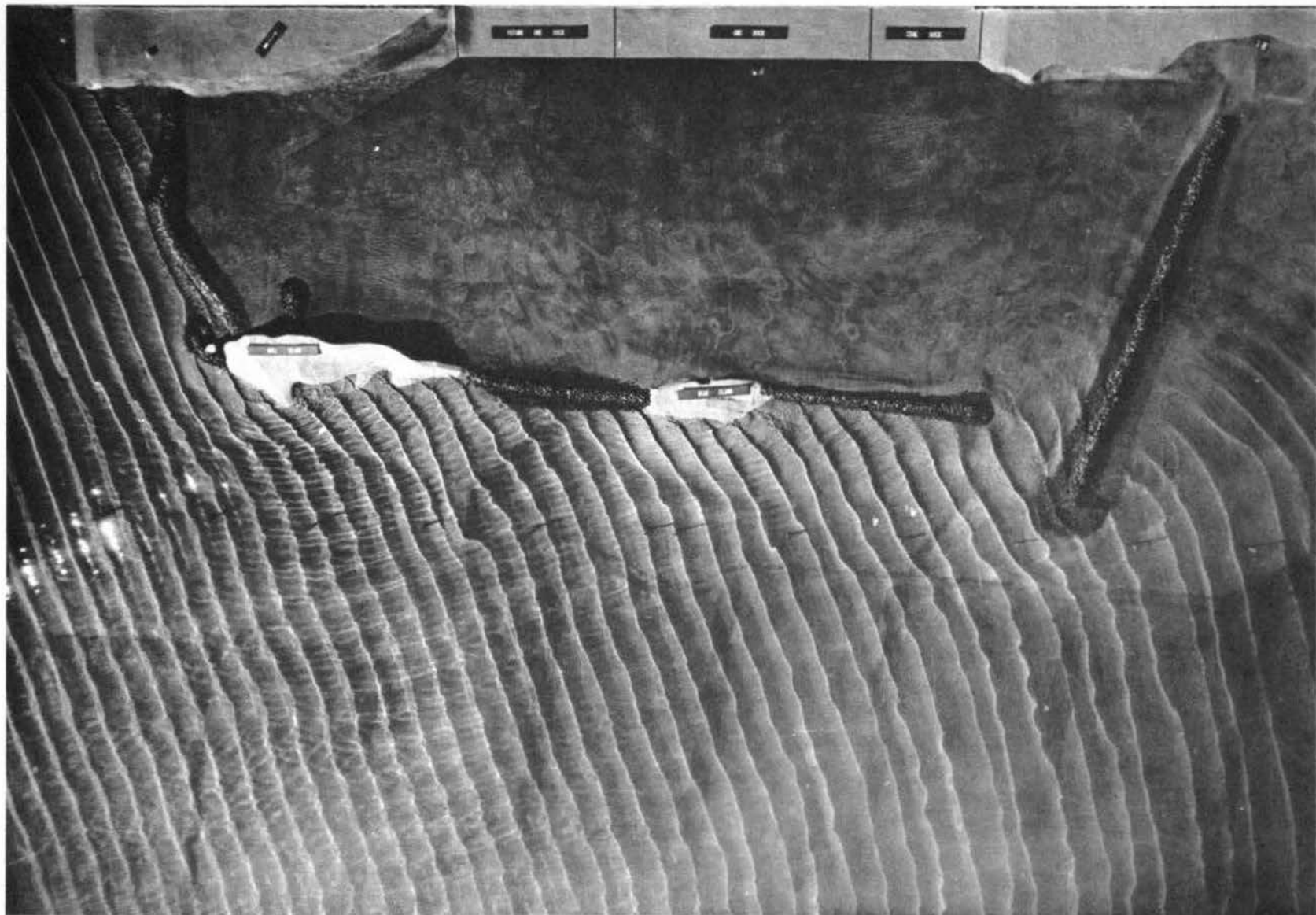
Photograph 29. Plan 2-E: 5.5-sec by 10-ft waves from S 22-1/2^{\circ} W
