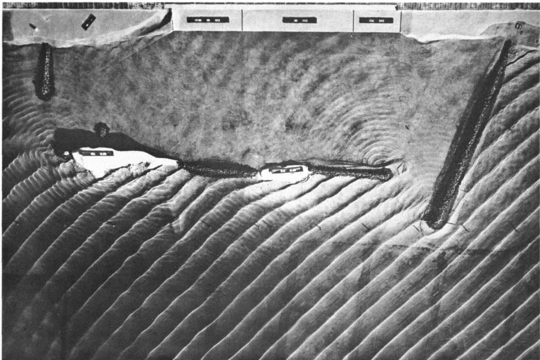
Photograph 10. Plan 1: 7.0-sec by 10-ft waves from N 82-1/2° E
