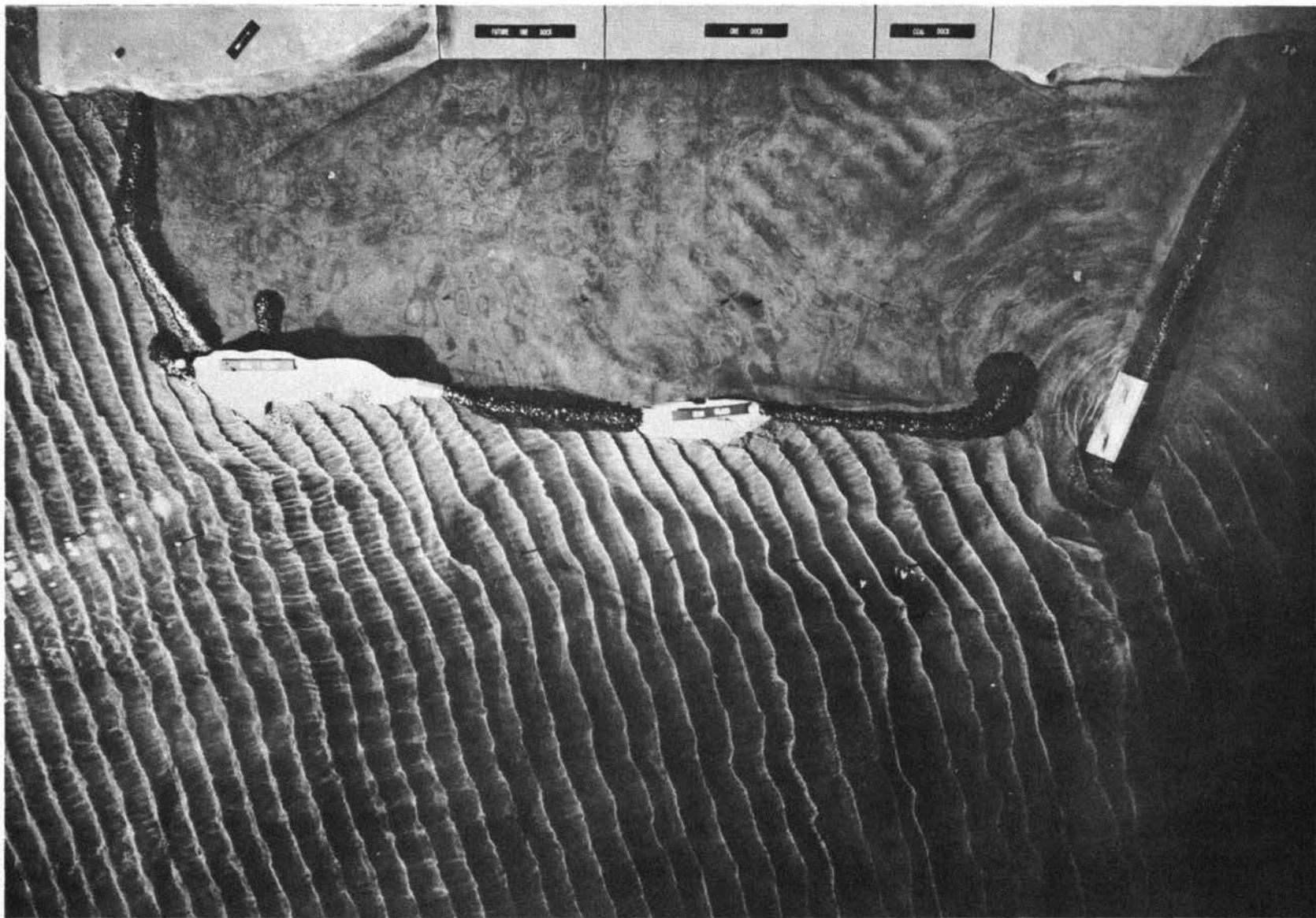
Photograph 32. Plan 3-ER: 5.5-sec by 10-ft waves from S 22-1/2^{\circ} W
