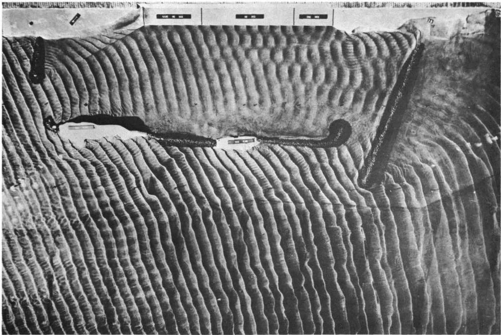
Photograph 14. Plan 5: 5.5-sec by 10-ft waves from S 22-1/2° W
