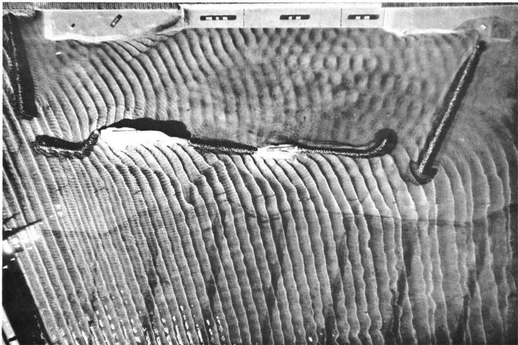
Photograph 17. Plan 8: 5.5-sec by 10-ft waves from S 22-1/2° W
