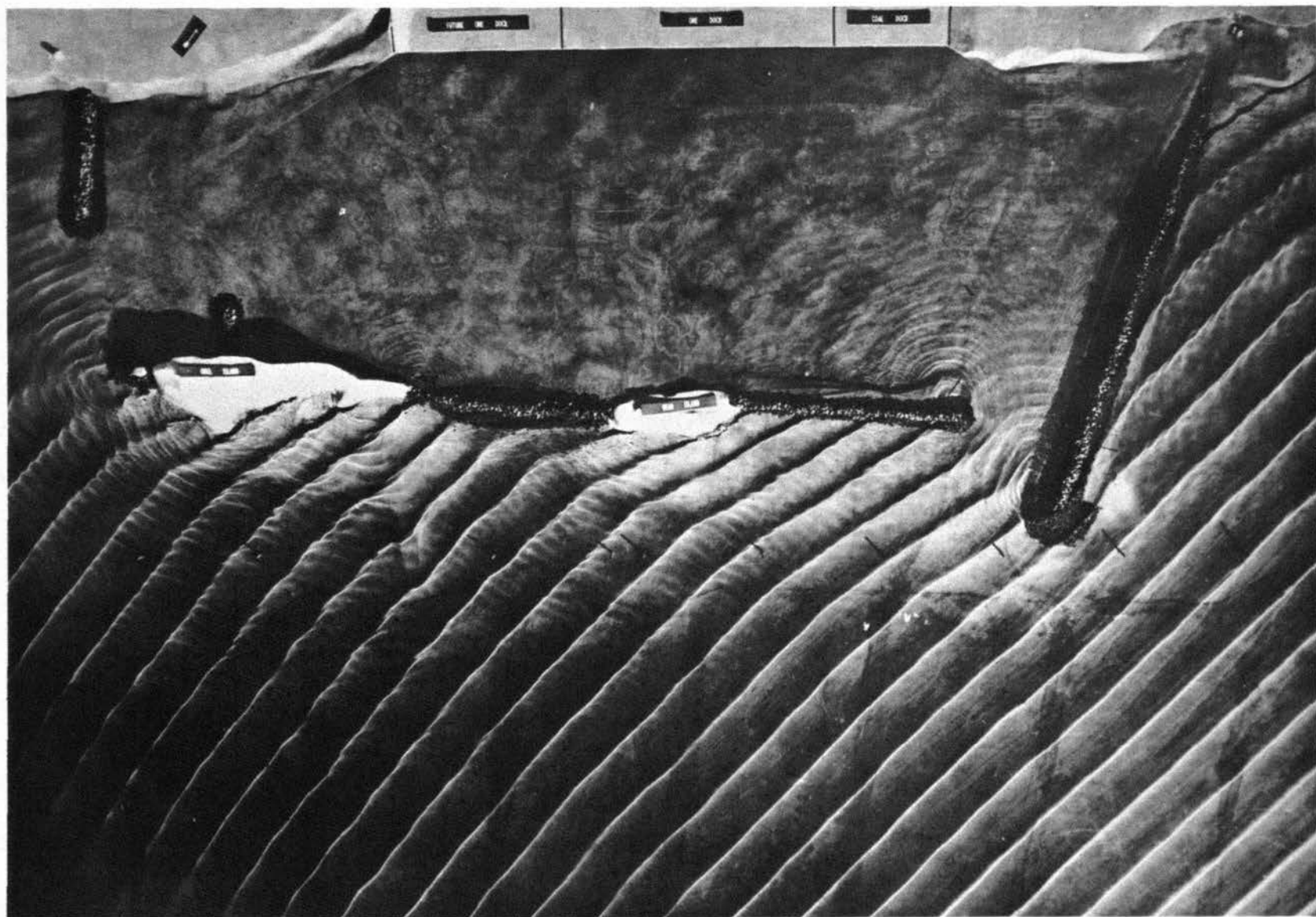
Photograph 11. Plan 2: 7.0-sec by 10-ft waves from N 82-1/2° E
