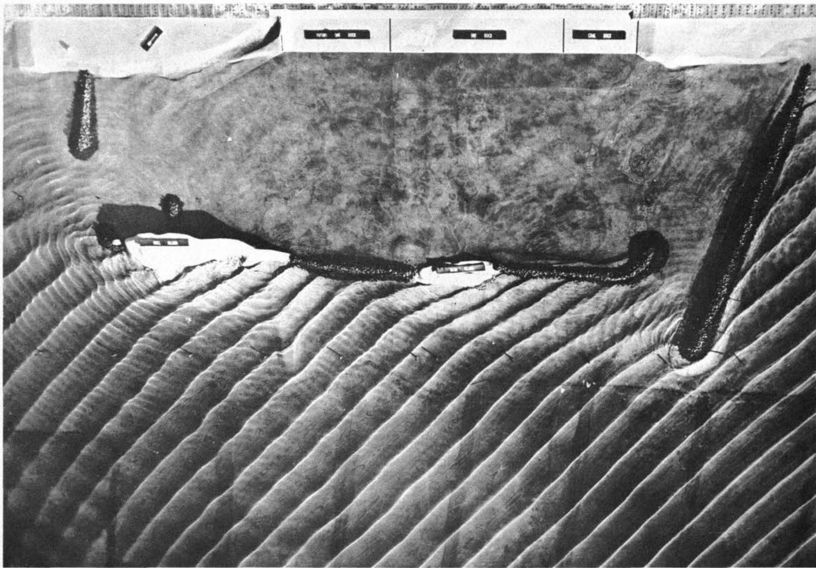
Photograph 4. Original plan: 7.0-sec by 10-ft waves from N 82-1/2° E
