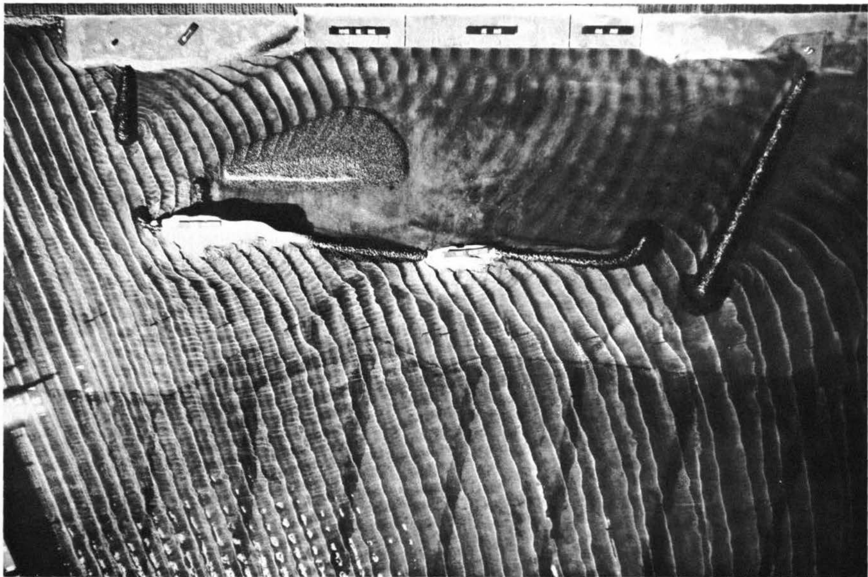
Photograph 20. Plan 11: 5.5-sec by 10-ft waves from S 22-1/2° W
