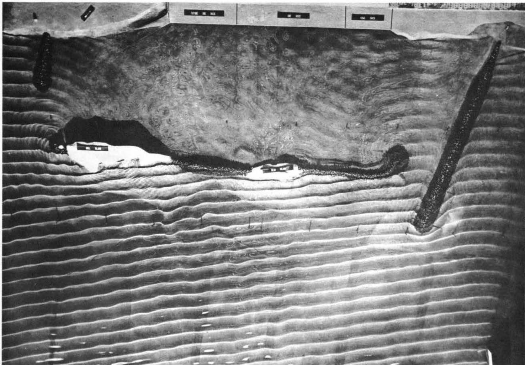
Photograph 5. Original plan: 5.5-sec by 7-ft waves from S 65° E
