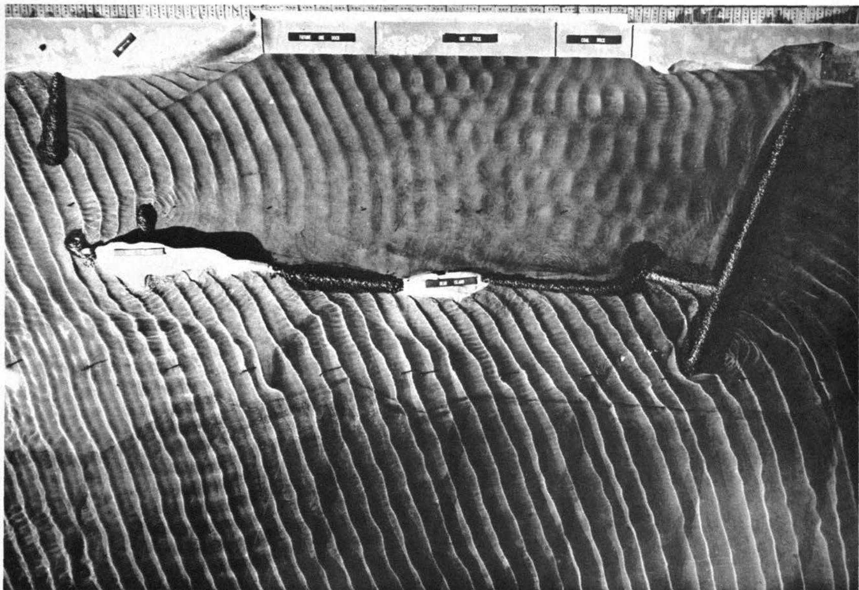
Photograph 9. Base-W: 5.5-sec by 10-ft waves from S 22-1/2^{\circ} W
