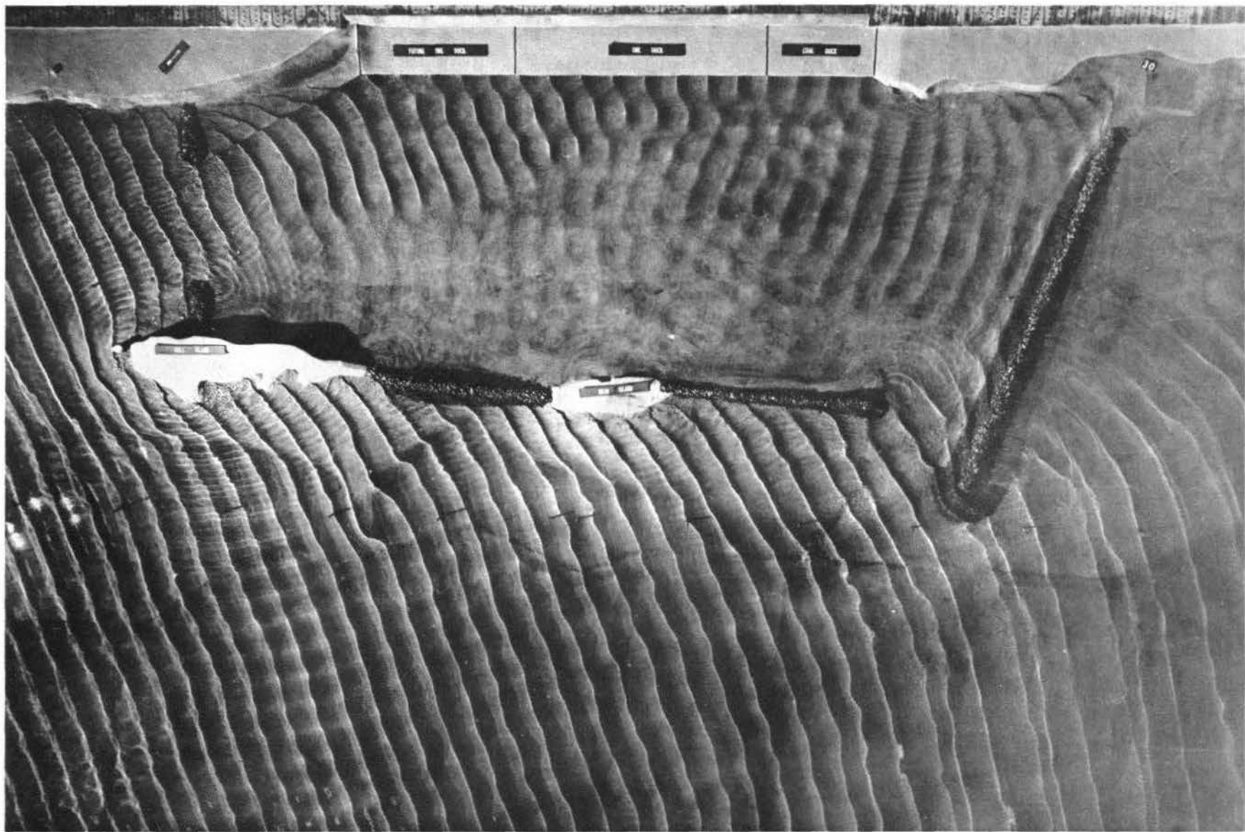
Photograph 24. Plan 13: 5.5-sec by 10-ft waves from S 22-1/2° W
