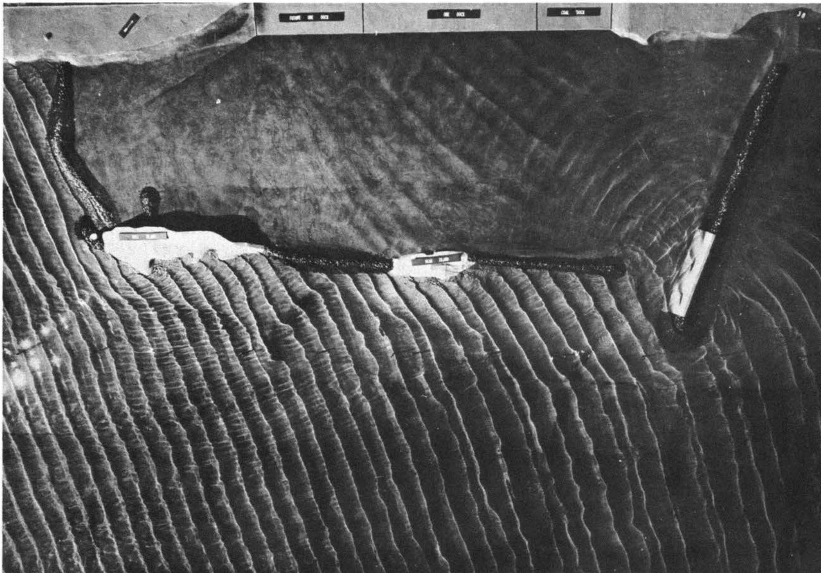
Photograph 30. Plan 2-ER: 5.5-sec by 10-ft waves from S 22-1/2° W
