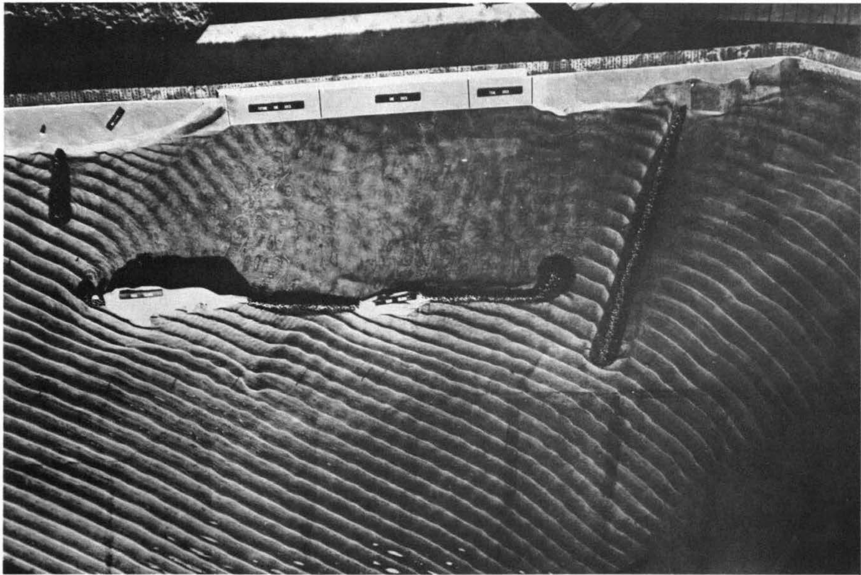
Photograph 6. Original plan: 5.5-sec by 7-ft waves from S 20° E
