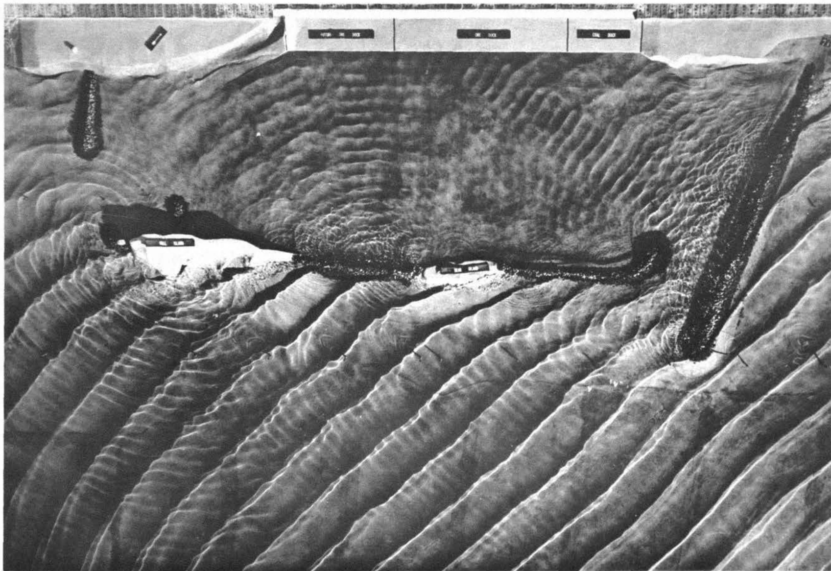
Photograph 3. Original plan: 8.5-sec by 20-ft waves from N 82\frac{1}{2}^{\circ} E
