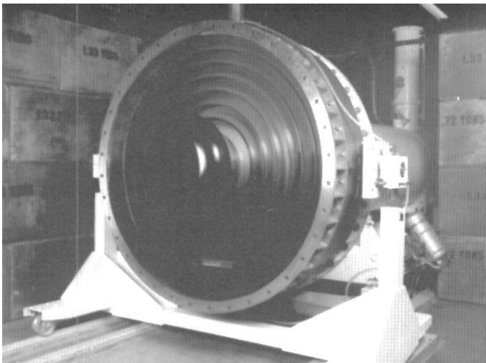
Fig. 3. REX Lucite insulator with grading rings.
