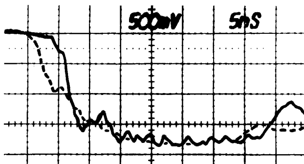
Fig. 11. Prepulse switch output, gaps set at 7.5 mm and closed (dotted trace). (0.82 MV/div, 5 ns/div)
