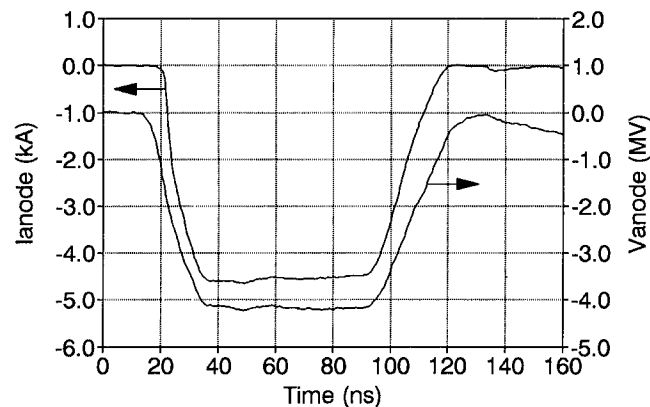
Fig. 7. REX A-K voltage and diode current for a 6-cm gap and a 6.35-cm-diam velvet cathode.
