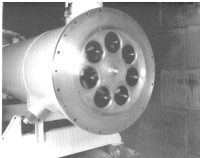
Fig. 12. Input end of OL2 showing output side of the 7-pin multichannel prepulse switch.
