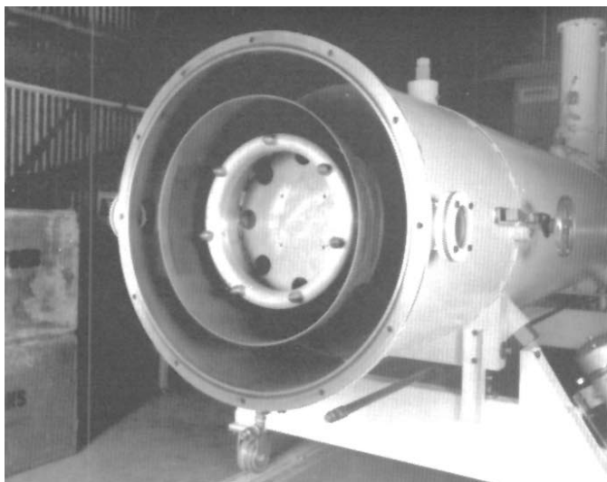
Fig. 10. Output end of OL1 showing the 7-pin, multi-channel prepulse switch and peaking section.
