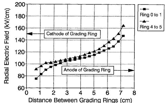
Fig. 6. Radial electric field across the surface of the most and least stressed insulator sections.
