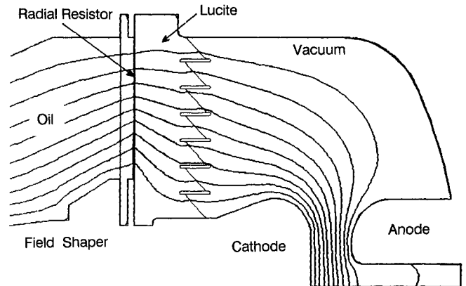
Fig. 4. Equipotential plot of vacuum vessel region.
