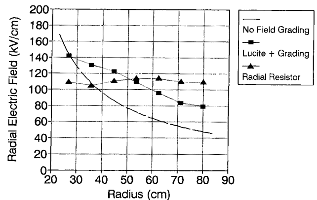
Fig. 5. Radial insulator electric field variation.
