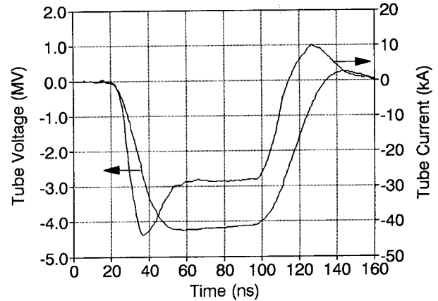
Fig. 8. REX pulsed-power drive for vacuum diode.
