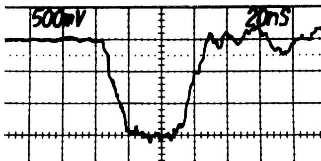
Fig. 13. REX Tube Voltage at 4 MV driving the 125- \Omega radial resistor as the load. (1.33 MV/div, 20 ns/div)
