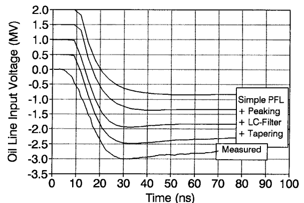
Fig. 9. Calculated waveforms showing the progressive shaping of the PFL output to drive OL1 as measured.
