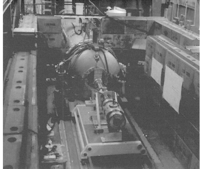
Fig. 2. REX experiment looking from the front end, showing the Marx generator in rear, transmission lines, dome-shaped vacuum vessel, and beam transport hardware.
