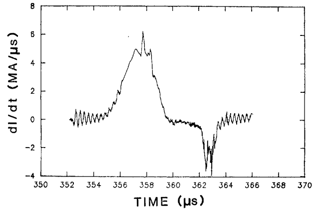
Fig. 10. Composite Faraday rotation and Rogowsky coil measurement of dI/dt in the vacuum region on Shot I. The positive spike indicates the rate of current transfer to the load, and the negative spike the effects of the pinch of gun plasma off the open end of the gun.
