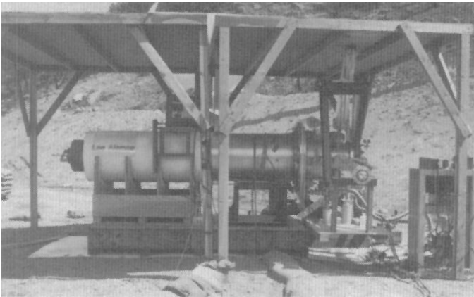
Fig. 1. A Procyon system ready to test. The three major sections are the MK-IX generator (left), the inductive store and opening switch (tri-axial center section), and the vacuum power flow section (right) seen with radiation diagnostic tubes attached.
