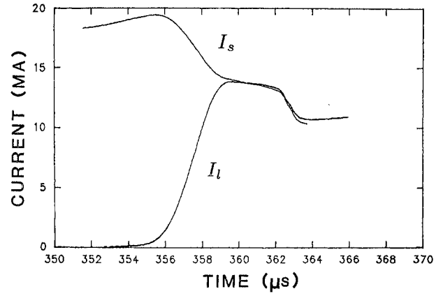
Fig. 9. I_s and I_l for Shot I, demonstrating total current transfer with a 10–90% risetime of <3 \mu\text{s} . In addition, the current drop at \sim 362 is due to the change in inductance as the plasma exits the gun and shows that the vacuum/dielectric interface and EFF have not failed.
