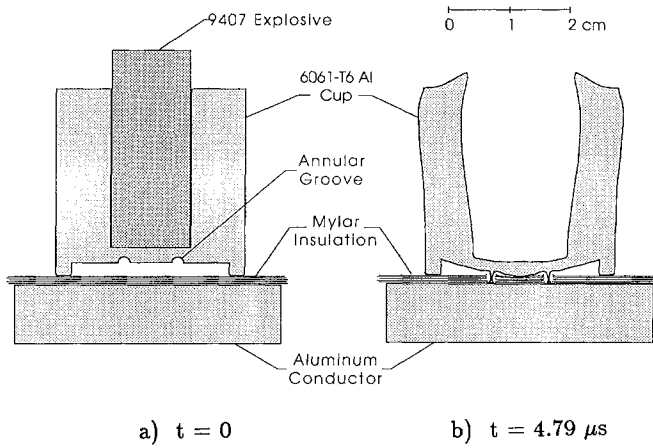
Fig. 6. Explosive-actuated closing switches used on Procyon tests. (a) cross-section of the initial configuration. (b) 2-D hydrodynamic code calculation showing the annular jet penetrating the Mylar insulation 4.79 \mu\text{s} after the explosive is detonated. Each test has six switches in parallel to provide symmetric current flow to the PFS.
