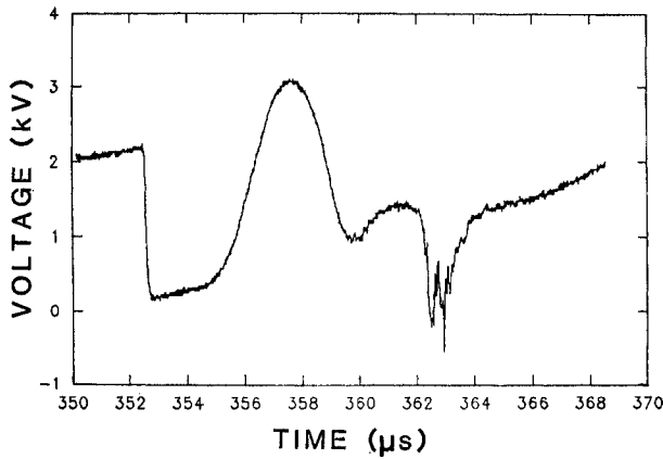
Fig. 7. Voltage across closing switches on Shot I. The abrupt break at 352.2 \mu\text{s} occurs when the switches close. The 3-kV positive spike at 358 and the negative spikes at 363 are features due to dI/dt and \sim 0.6\text{-nH} circuit inductance inside the voltage probe loop. The resistance of the switches at 360 \mu\text{s} is \sim 0.08 \text{ m}\Omega .
