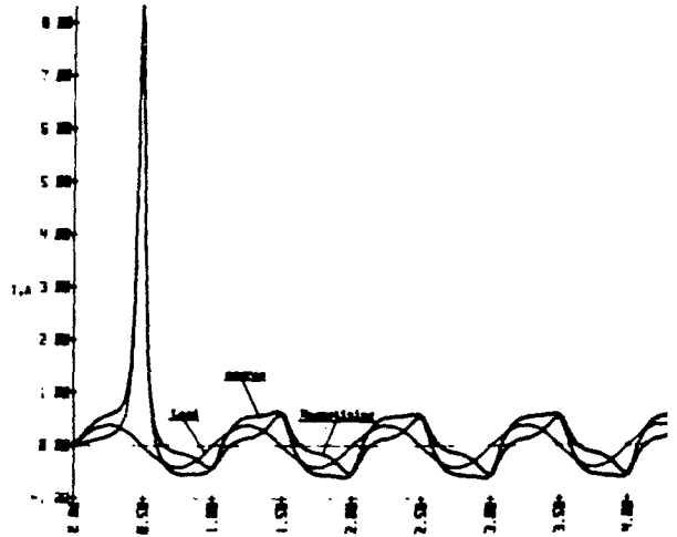
Currents in a Lumped Parameter Transformer Model
