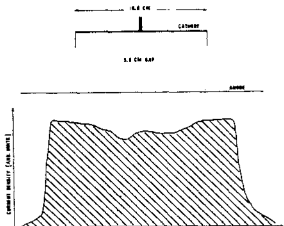
Figure 4. Beam profile at anode along Z-axis.
