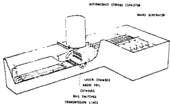
Figure 5 Modular accelerator for laser excitation using radial e-beams.
