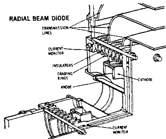
Figure 2. Reble Diode
