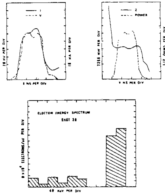
Figure 3 Typical diode waveforms. The voltage waveform has been corrected for the inductive contribution. The electron spectrum was obtained by un- folding the voltage and current waveforms.
