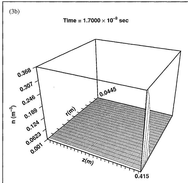
Figure 3. Appearance of electron density due to field emission at the flat end plate: (a) axial field; (b) electron density.
