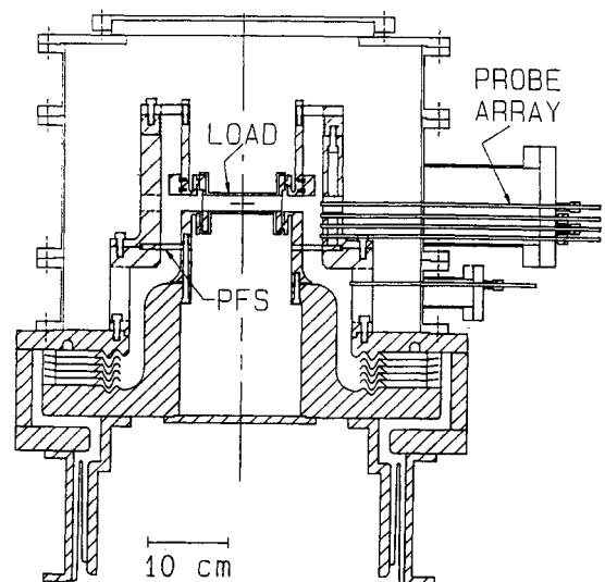
Fig. 2. PFS installed in the power flow channel.
