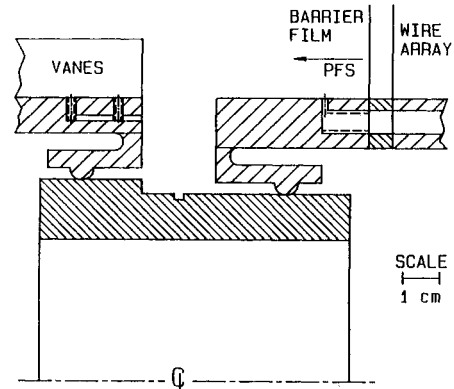
Fig. 1. Plasma flow switch schematic.
